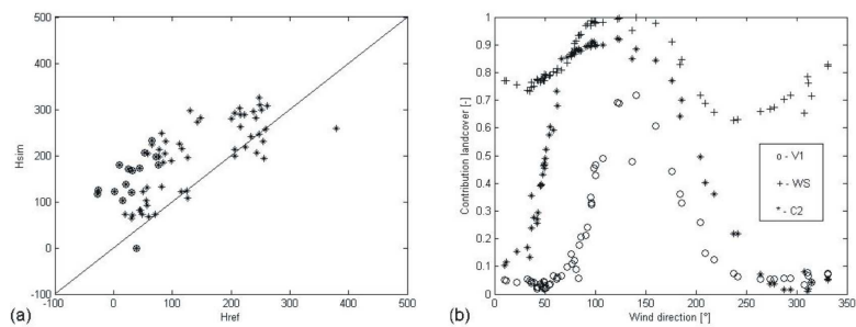
Fig. 4. Simulated versus reference fluxes, assuming known ratio of component fluxes. Influence of atmospheric stability contrast, stable by circles (a) , homogeneity of sonic footprints related to wind direction (b) .
