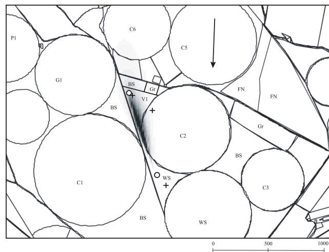
Fig. 2. Map (north oriented) of the experimental set-up at the Las Tiasas experimental farm, showing landcover units and scintillometer weighted observation source area. The LAS is represented by two white circles, and the sonic anemometers by (three) crosses, whereas an arrow indicates the wind direction. Letters represent landcovers vineyard (“V”), grass (“Gr”), corn (“C”), bare soil (“BS”), garlic (“G”), potato (“P”) and forest nursery (“FN”), whereas the numbers refer to the respective field numbers.
