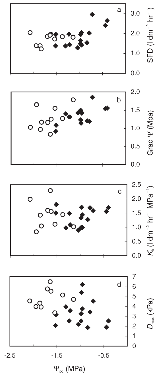
Figure 6. Plots of predawn leaf water potential ( \Psi_{pd} ) versus (a) daily maximum sap flow density per sapwood area (SFD), (b) maximum gradient of leaf water potential (grad \Psi ), (c) whole hydraulic conductivity ( K_h ) and (d) maximum vapor pressure deficit of the air ( D_{max} ). Measurements were made for the full canopy stages during wet (◆; August–September, n = 16 ) and dry seasons (○; October–January, n = 10 ).
