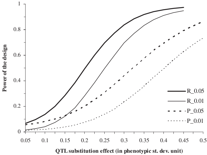
Figure 1. Approximate power of the design for the detection of QTL for production traits and reproduction traits, as a function of the QTL substitution effect. R_0.05 and R_0.01 are, respectively, the power for a 0.1 heritability reproduction trait considering a 5% or a 1% type I error. P_0.05 and P_0.01 are, respectively, the power for a 0.4 heritability production trait considering a 5% or a 1% type I error.
