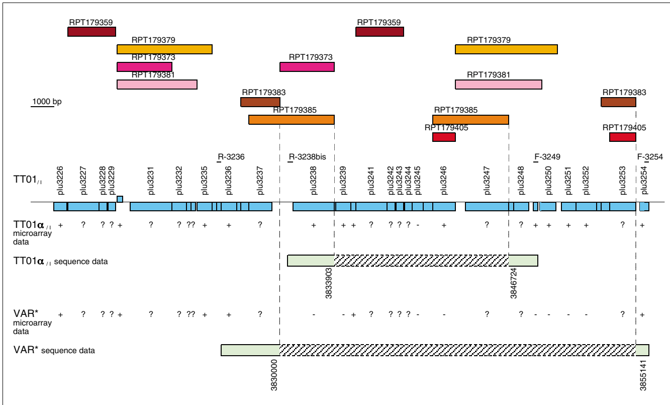
Figure 5 Successive deletions between homologous repeats in the region H. Genetic map of TT01 fl region H is shown (blue boxes are open reading frames [ORFs]). Location of repetition units (RPT) larger than 1 kilobase (kb) is indicated (hatched colored boxes). RPT were systematically searched on the whole TT01 fl genome sequence by using Nosferatu, software that can detect approximate repeat sequences [46]. The RPTs are numbered according their position on the chromosome. DNA microarray data for the TT01 fl and VAR* genomes are indicated. '+': the gene is present. '-': the gene is absent. '?': the gene is not represented on the microarray. Schematic representation of TT01 fl and the VAR* variant deletions is shown. Deletion borders were obtained from sequencing between the R-3236 and F-3254 primers in the VAR* variant, and between the R-3238bis and F-3249 primers in the TT01 fl variant. Green and hatched gray boxes represent regions in TT01 fl and VAR* genomes variants that were found to be present or absent, respectively. The deleted regions encompassed sequence between coordinates 3.833.904 and 3.846.724 in TT01 fl genome and coordinates 3.830.001 and 3.855.141 in VAR* genome.
