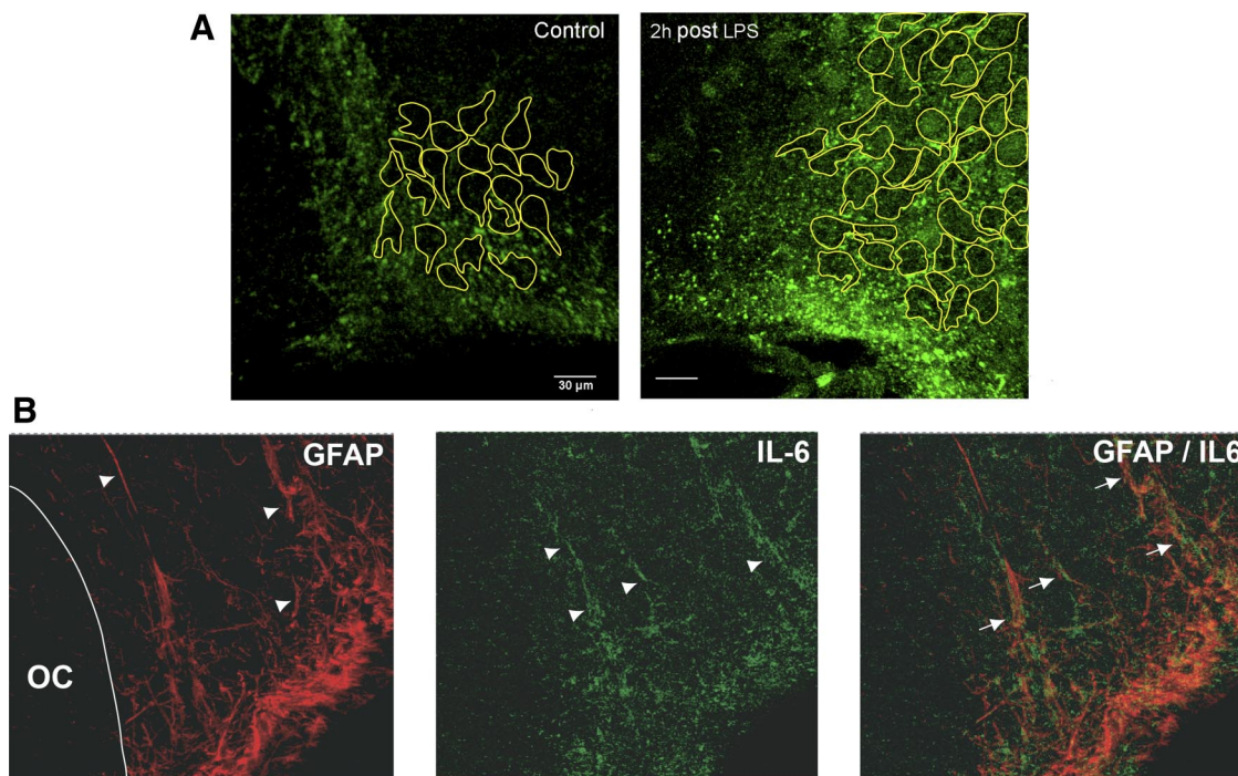
Fig. 7. IL-6 protein expression is increased in SON in response to immune challenge and expressed by astrocytes. Rats were injected ip with PBS ( n = 3 ) or LPS ( n = 3 ) and euthanized 2 h later to perform single-fluorescent staining of IL-6 (A; scale bar = 40 μm) or double-fluorescent staining of IL-6 and glial fibrillary acidic protein (GFAP) in the SON of LPS-treated rats (B; scale bar = 30 μm), followed by analysis on a confocal microscope.
