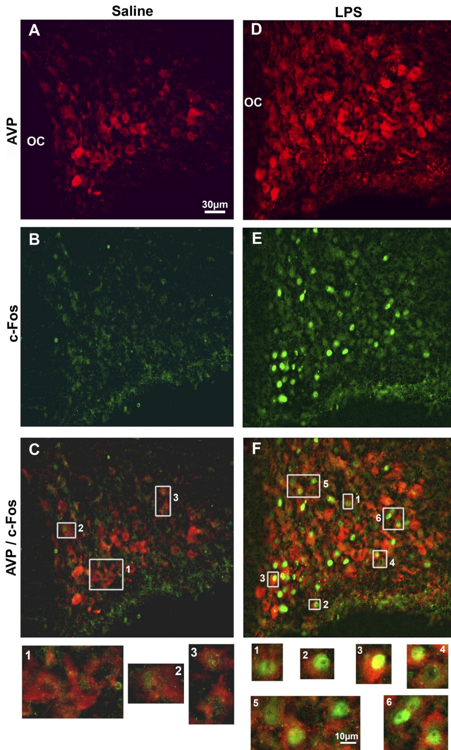
Fig. 2. Expression of c-Fos in AVP neurons of the SON 1 h post-LPS injection. A and D : immunohistochemistry of AVP in control and LPS-treated rats. B and E : immunohistochemistry of c-Fos in control and LPS-treated rats. C and F : merge of A and B and D and E showing colocalization of Fos positive nuclei in AVP positive neurons (scale bar = 30 \mu m). Compared with control, Fos protein expression was dramatically increased 1 h post-LPS treatment ( n = 3 /group) and expressed in numerous labeled AVP neurons. Boxed areas in C and F are numbered and enlarged below with scale bars. OC, optic chiasma; AVP, arginine vasopressin.
