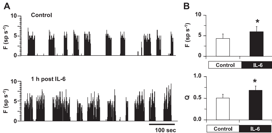
Fig. 9. Brain injection of IL-6 increases electrical activity of AVP neurons. Adult rats were anesthetized, and AVP neuron electrical activity was recorded by electrophysiology in SON. A : discontinuous recordings showing the evolution of an AVP neuron electrical activity recorded before and 1 h after icv IL-6 injection. The frequency, F , is expressed in spikes/s. B : histograms of the averaged values of the frequency of discharge, F ( n = 5 , repeated-measures ANOVA; *P < 0.05 ), and the activity quotient, Q ( n = 5 , repeated-measures ANOVA; *P < 0.05 ). Each neuron was its own control.
