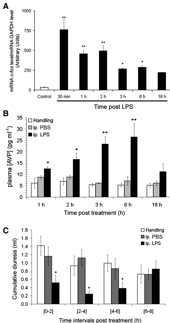
Fig. 1. Rapid and sustained activation of arginine vasopressin (AVP) neurons in supraoptic nucleus (SON) after lipopolysaccharide (LPS) treatment. A: using real-time PCR, mRNA c-fos level was quantified and normalized to mRNA GAPDH level (arbitrary units) in control (1 h post-PBS injection) and in LPS-treated rats at different times postinjection (30 min, 1 h, 2 h, 3 h, 6 h, and 18 h) ( n = 3 /group). Compared with control, LPS treatment increased mRNA c-fos level with time (ANOVA followed by Student-Newman-Keuls post hoc test: * P < 0.05 and ** P < 0.01 ). B: using specific competitive binding assay, AVP concentration (pg/ml) was measured in plasma of handled, PBS-treated, and LPS-treated rats at different times posttreatment (1, 2, 3, 6, and 18 h) (see METHODS for n /group). Compared with handling and PBS treatment, LPS injection increased plasma AVP release with time (ANOVA followed by Student-Newman-Keuls post hoc test: * P < 0.05 and ** P < 0.01 ). C: cumulative urine flow (diuresis, ml) was measured in handled, PBS-treated, and LPS-treated rats every 2-h period after treatment between 1000 and 1800. Animals were individually housed in a metabolic cage, and each one was its own handled and PBS-treated control ( n = 10 /group). Compared with handling and PBS treatment, LPS injection decreased urine flow volume with time (ANOVA followed by Student-Newman-Keuls post hoc test: * P < 0.05 ). ip, Intraperitoneal.
