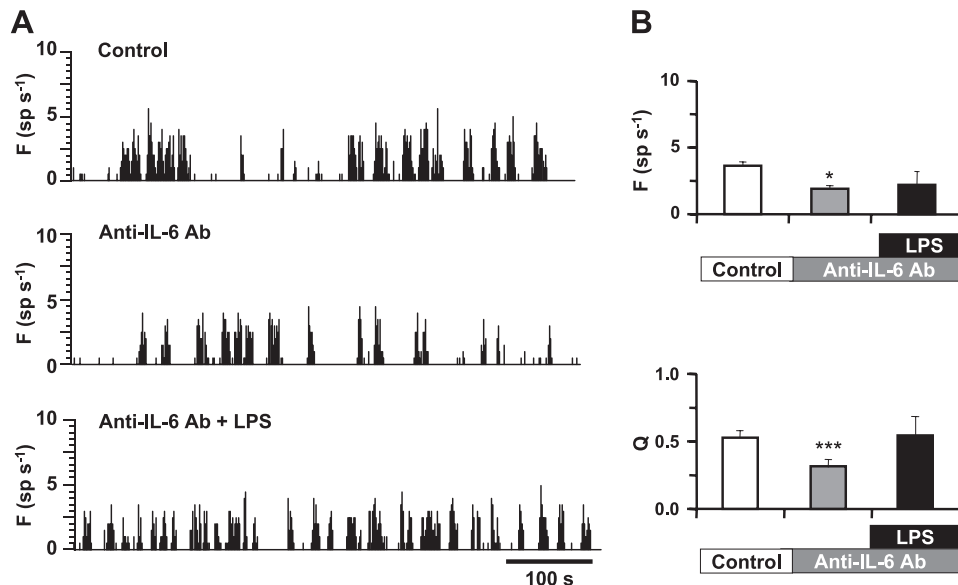
Fig. 8. IL-6 neutralizing antibodies blocked LPS-induced AVP neurons electrical activation. Adult rats were anesthetized, and AVP neuron electrical activity was recorded by electrophysiology. A: discontinuous recordings showing the evolution of AVP neuron electrical activity before (control) and after intracerebroventricular (icv) injection of IL-6 neutralizing antibodies. Forty minutes after the IL-6 neutralizing antibody treatment, LPS was ip injected and the electrical activity of the same AVP neuron further recorded for 1 h. The frequency, F , is expressed in spikes/s. B: histograms of the averaged values of the frequency of discharge F ( n = 6 , repeated-measures ANOVA; *P < 0.05 , IL-6 neutralizing antibodies vs. control) and the activity quotient Q ( n = 6 , repeated-measures ANOVA; *P < 0.001 , IL-6 neutralizing antibodies vs. control). Each neuron was its own control.
