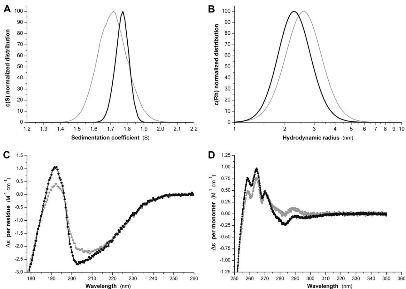
Fig. 2. Analysis of GarA (gray lines) and GarA \Delta pT22 (black lines) by AUC, DLS and CD. (A) Sedimentation coefficient distributions obtained by sedimentation velocity AUC experiments. (B) Hydrodynamic radius distributions obtained from DLS experiments. (C) Far-UV CD spectra of the two proteins. (D) Near-UV CD spectra of the two proteins.
