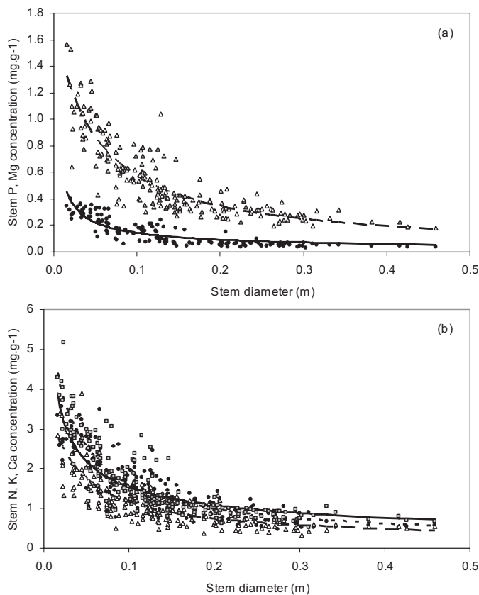
Figure 3. Relationships between nutrient concentration ( \text{mg g}^{-1} ) of the stem (all stem tissues combined) of an annual shoot and the stem diameter (m) of the same annual shoot. (a) Measured P concentration = closed circle; measured Mg concentration = open triangle; regression function for P = solid line; regression function for Mg = dashed line. (b) Measured N concentration = closed circle; measured K concentration = open triangle; measured Ca concentration = grey square; regression function for N = solid line; regression function for K = dashed line; regression function for Ca = dotted line. The parameters of the regression functions are summarized in Table III.
