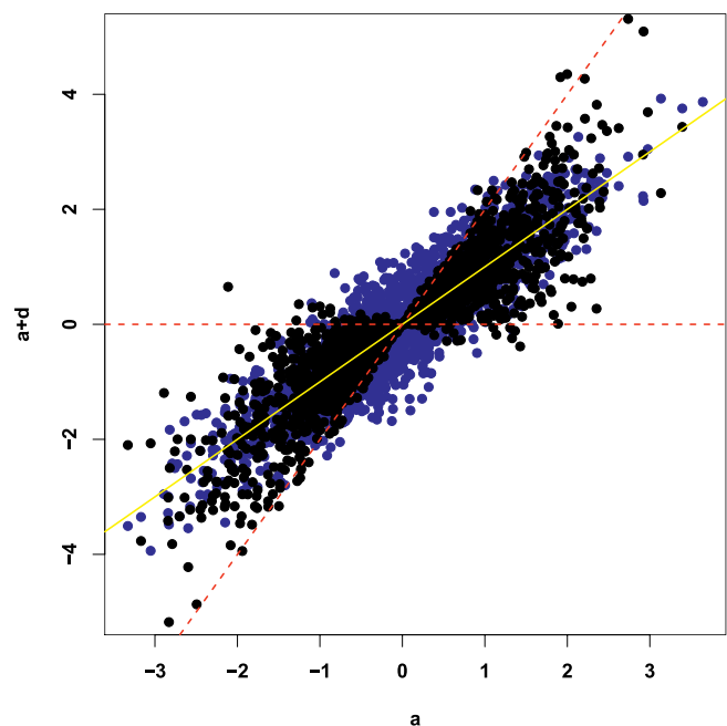
Figure 5. Scatter Plot of Samples from Prior Distribution of a (x-axis) and a + d (y-axis), for Priors D_1 (Black) and D_2 (Blue)
