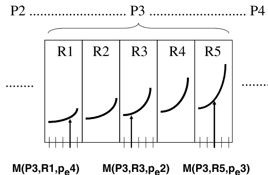
Figure 9. Two-dimensional representation of the 5-D problem in (M, P, R, p_s, p_e) used for spatially homogeneous parametric configurations: P, R, p_s and/or p_e values are placed on the x ordinate, and only M appears in the y ordinate.
