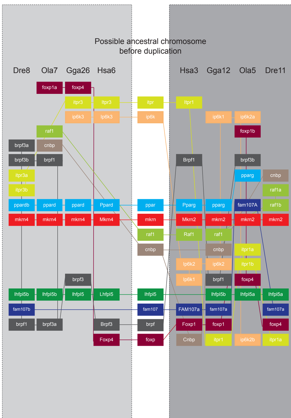
Figure 3 Mkrn2 and mkrn4 are included in large paralogs in bony vertebrates. Genes are indicated in colored boxes. Colored lines connect orthologs on one side with paralogs on the other side of the figure. Each grey panel contains a set of orthologous syntenic regions, the putative ancestral region before duplication is shown in the central white panel. Dre: Danio rerio (zebrafish); Gga: Gallus gallus (chicken); Hsa: Homo sapiens (human); Ola: Oryzias latipes (medaka fish). Accession numbers of genes presented in this figure are listed in Additional file 2.
