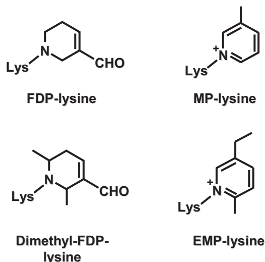
Figure 4. Lysine adducts.
