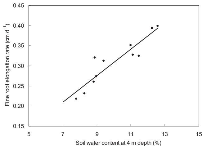
Figure 3. Relationship between the monthly average root elongation rate (eight rhizotrons) and soil water content at a depth of 4 m in the 2-year-old stand. The linear relationship was significant ( r = 0.93 ).
