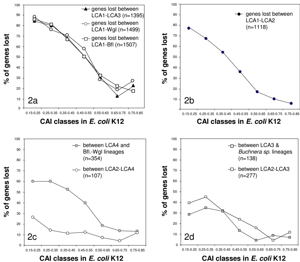
Figure 2 Relationship between frequency of gene loss in endosymbionts and adaptive codon bias (CAI) of the E. coli ortholog at different depths of the tree. y-axis: percentages of genes lost at least on one occasion between different nodes (or a node and a tip), x-axis: CAI classes of E. coli K12.
