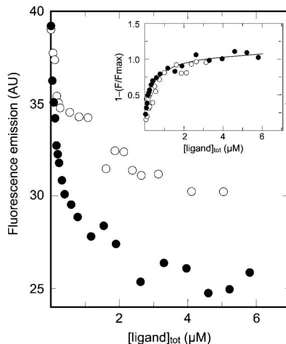
Fig. 2. Spectroscopic characterization of the interaction between eIF4E and VPg. eIF4E tryptophan fluorescence was measured following the addition of VPg ( \circ ) or VPg-CD ( \bullet ) ( 0.05 – 5 \mu\text{M} ) was added to a 2.5 \mu\text{M} eIF4E solution in 1 ml of 20 mM HEPES/KOH (pH 7.6), 25 mM KCl, 1 mM DTT, 10 % glycerol. The mixture was incubated (5 min at 25 \text{ }^\circ\text{C} ) until a steady-state fluorescence at 342 nm was reached upon excitation at 280 nm. AU, arbitrary units. Inset: variation of eIF4E fluorescence as a function of increasing concentrations of VPg ( \circ ) or VPg-CD ( \bullet ).
