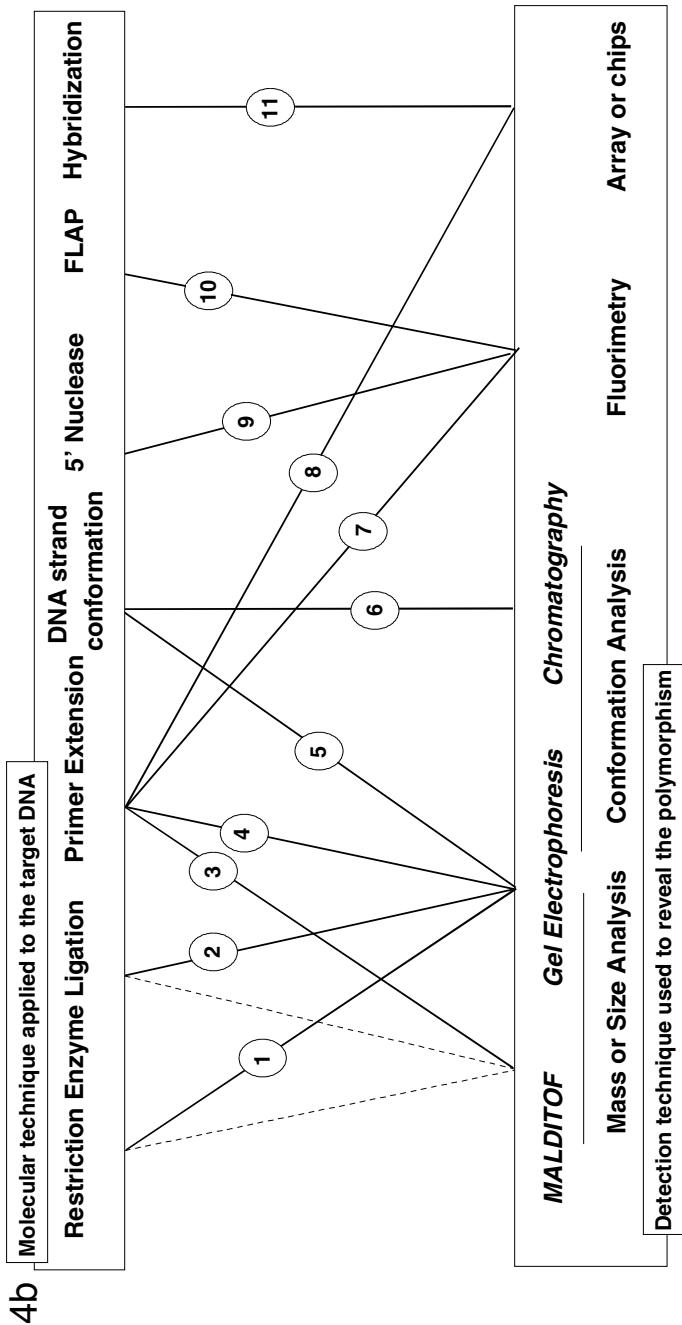
Figure 4. SNP genotyping techniques. 4a: principal molecular reactions used to generate allele-specific signals. 4b: links between the signal generation and detection. The reason for the broad range of techniques available appears clearly, since many of the products generated by the allele-specific reactions can be detected with different methods. 1 : PCR/FLP, 2 : LAR or OLA, 3 : Good Assay, 4 : Minisequencing techniques, Snapshot ..., 5 : SSCP or DGGE, 6 : DHPLC, 7 : Pyrosequencing, READit, 8 : SNP it, 9 : Taqman, 10 : Invader Assay, 11 : Microarray or DNA chips
