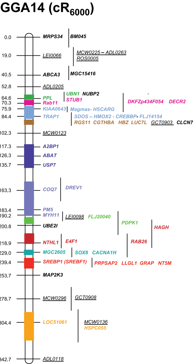
Figure 3. Comparative mapping between the GGA14 RH map and the sequence maps of human regions HSA16p13.3 and HSA17p11.2. Markers localised on the genetic map are underlined on the RH map. Groups of global conserved gene order between chickens and humans are identified by coloured boxes. Genes or EST markers that could not be assigned to any such group are in black.
