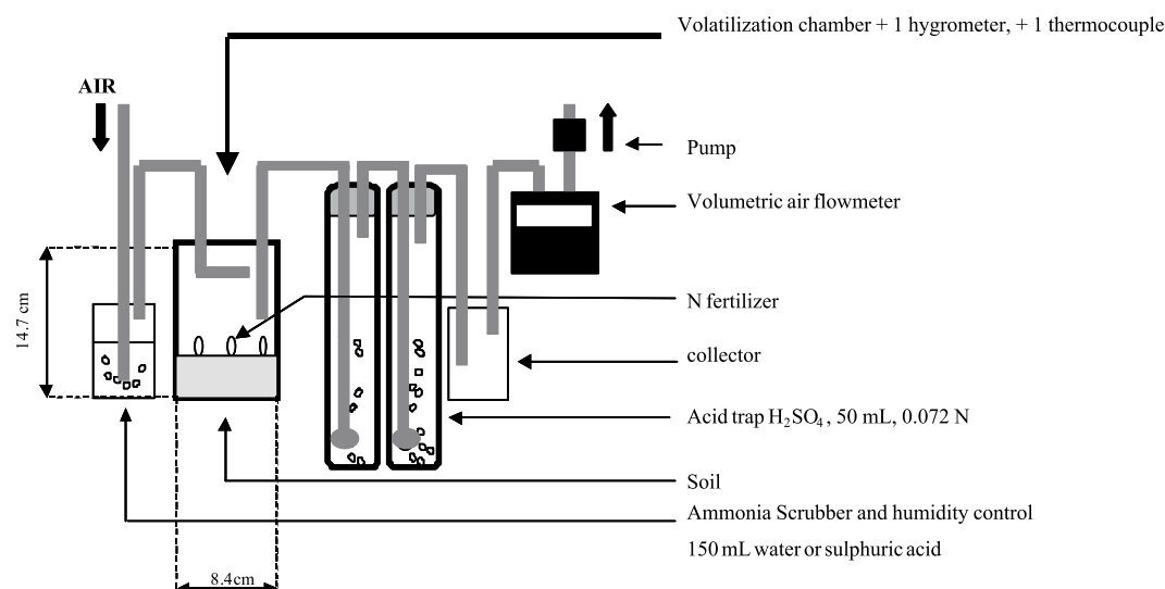
Figure 1. Schema of the volatilization chamber.
