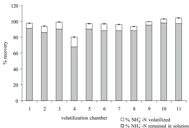
Figure 3. Efficiency of the 11 volatilization chamber system. Vertical bars represent the measurement deviation (7%).
