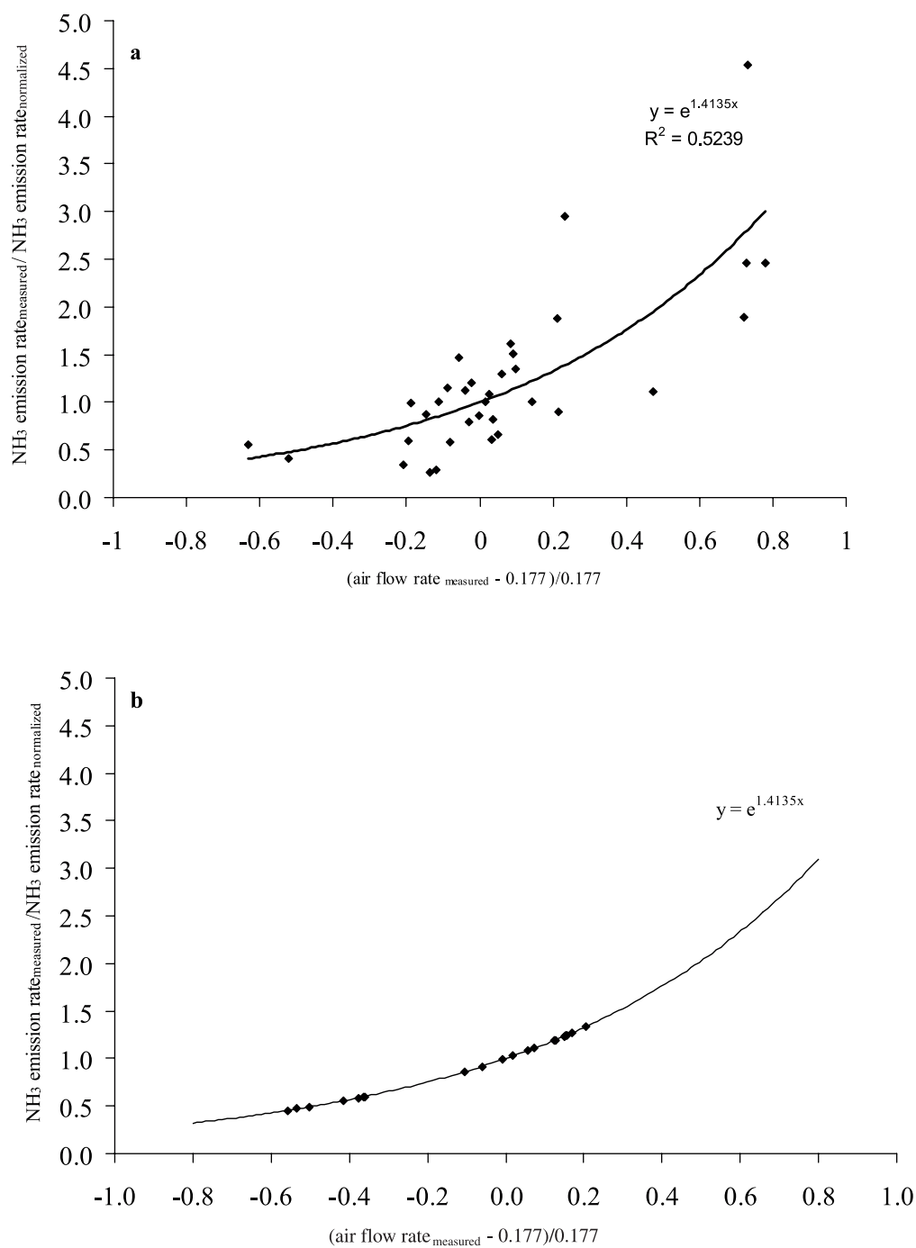
Figure 2. Effect of the air flow rate on NH 3 emission (a) and after normalization (b).
