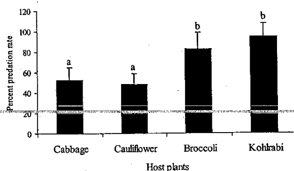
Fig. 1. The effect of the presence of DBM larvae on the predation rate by larvae of C. carnea . Bars with the same letters are not significantly different ( P < 0.05 ; repeated measure ANOVA); mean number \pm SE obtained from 20 replications, each replicate consists of 10 insects.
