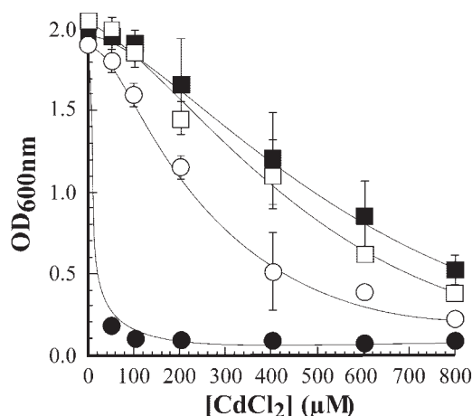
FIG. 10. Effect of heterologously expressed wild-type and Ser-to-Ala mutant-substituted AtPCS1-FLAG on the Cd 2+ hypersensitivity of mutant S. cerevisiae ycf1Δ strain DTY167. Strain DTY167 was transformed with the pYES3-AtPCS1-FLAG vector encoding wild-type AtPCS1 (○) or mutant AtPCS1 in which the Ser residue at position 21 (□) or 164 (■) was singly substituted with Ala or with the empty pYES3 vector (●). Cd 2+ hypersensitivity was assessed as described in the legend to Fig. 9.
