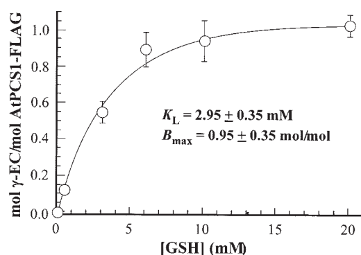
FIG. 4. Concentration dependence of \gamma -glutamylcysteinylolation of AtPCS1-FLAG by GSH. Aliquots of purified AtPCS1-FLAG (27.3 \mu g) were incubated for 10 min with the indicated concentrations of [ ^{35} S]Cys-labeled GSH in 100 mM HEPES/BTP buffer (pH 8.0). After termination of the reaction by the addition of 100 mM sodium acetate buffer (pH 4.0) containing 6 M guanidine HCl, radioactivity associated with the enzyme was determined by membrane filter binding and liquid scintillation counting. The radiocorporation data were fitted to a rectangular hyperbola, and the concentrations of GSH required for half-maximal ( K_L ) and maximal ( B_{\max} ) labeling were estimated by nonlinear least-squares analysis (40). Values shown are means \pm S.E. ( n = 3-5 ).
