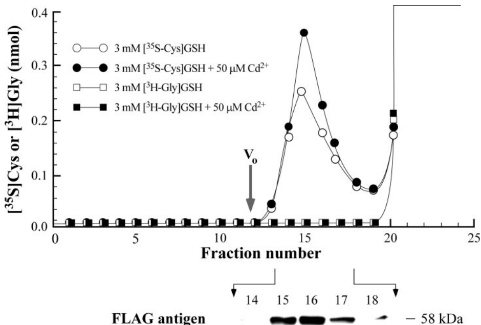
FIG. 2. Synthesis of \text{PC}_3 from \text{PC}_2 and radiolabeled GSH. At the outset, the reaction medium contained 1 mM GSH, 100 \mu\text{M} \text{PC}_2 , 10 \mu\text{M} \text{CdCl}_2 , 1 \mu\text{g} AtPCS1-FLAG, and 6 \mu\text{Ci} of either [ ^{35}\text{S} ]Cys-labeled GSH or [ ^3\text{H} ]Gly-labeled GSH. At the times indicated, \text{PC}_2 (●) and \text{PC}_3 (○) were separated by RP-HPLC and quantitated as thiol equivalents by reaction with DTNB. Radioactivity was determined by liquid scintillation counting. Numbers labeled [ ^3\text{H} ]Gly/ \text{PC}_2 and [ ^3\text{H} ]Gly/ \text{PC}_3 denote moles of [ ^3\text{H} ]Gly per \text{PC}_2 or \text{PC}_3 molecule, respectively; numbers labeled [ ^{35}\text{S} ]Cys/Cys in \text{PC}_3 denote moles of [ ^{35}\text{S} ]Cys per mole of Cys in \text{PC}_3 . Values shown are means \pm S.E. ( n = 3-5 ).
