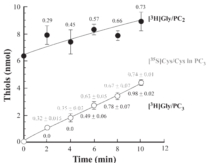
FIG. 2. Synthesis of \text{PC}_3 from \text{PC}_2 and radiolabeled GSH. At the outset, the reaction medium contained 1 mM GSH, 100 \mu\text{M} \text{PC}_2 , 10 \mu\text{M} \text{CdCl}_2 , 1 \mu\text{g} AtPCS1-FLAG, and 6 \mu\text{Ci} of either [ ^{35}\text{S} ]Cys-labeled GSH or [ ^3\text{H} ]Gly-labeled GSH. At the times indicated, \text{PC}_2 (●) and \text{PC}_3 (○) were separated by RP-HPLC and quantitated as thiol equivalents by reaction with DTNB. Radioactivity was determined by liquid scintillation counting. Numbers labeled [ ^3\text{H} ]Gly/ \text{PC}_2 and [ ^3\text{H} ]Gly/ \text{PC}_3 denote moles of [ ^3\text{H} ]Gly per \text{PC}_2 or \text{PC}_3 molecule, respectively; numbers labeled [ ^{35}\text{S} ]Cys/Cys in \text{PC}_3 denote moles of [ ^{35}\text{S} ]Cys per mole of Cys in \text{PC}_3 . Values shown are means \pm S.E. ( n = 3-5 ).
