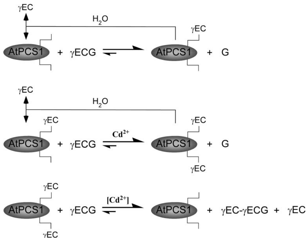
FIG. 7. Tentative model for the multisite \gamma -Glu-Cys acylation of AtPCS1 concomitant with the generation of free Gly, \gamma -Glu-Cys, and PC 2 . The first step is the Cd 2+ -independent formation of enzyme acylated with \gamma -Glu-Cys at one site coincident with the cleavage of Gly from the first molecule of GSH. The second step is the Cd 2+ -dependent (or blocked thiol-dependent) \gamma -Glu-Cys acylation of the enzyme at a second site coincident with the cleavage of Gly from a second molecule of GSH (or PC n ). In the third step, which may or may not depend on the provision of Cd 2+ (or a thiol peptide with a blocked thiol group), one of the \gamma -Glu-Cys units from the disubstituted enzyme intermediate is transferred to a third molecule of GSH (or PC n ) to generate the product, PC 2 (or PC n+1 ) containing one additional \gamma -Glu-Cys repeat. In all three steps, one or more of the \gamma -Glu-Cys acyl-enzyme intermediates can undergo uncoupled hydrolysis to liberate \gamma -Glu-Cys and to yield free Gly in excess of the amount specifically required for PC chain extension. In the third step, the simple transfer of one of the two enzyme \gamma -Glu-Cys acyl groups to water is considered to contribute to the free energy input required for the formation of a new Cys-Glu peptide bond between the other enzyme-bound \gamma -Glu-Cys unit and GSH (or PC n ) in the PC 2 (or PC n+1 ) product.
