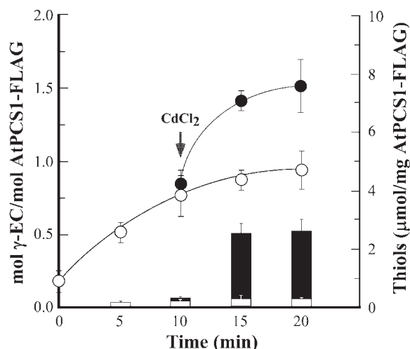
FIG. 5. Time dependence of acylation of AtPCS1-FLAG by GSH and net synthesis of PCs in the absence ( \circ ) or presence ( \bullet ) of 50 \mu M \text{CdCl}_2 . Aliquots of purified AtPCS1-FLAG (27.3 \mu g) were incubated with [ ^{35} S]Cys-labeled GSH (3 mM) in 100 mM HEPES/BTP buffer (pH 8.0) lacking \text{CdCl}_2 throughout the 20-min incubation period ( \circ ) or for 10 min before and 10 min after the addition of \text{CdCl}_2 (50 \mu M) ( \bullet ). At the times indicated, the reactions were terminated, and the amount of ^{35}\text{S} label (as \gamma -Glu-Cys) incorporated into AtPCS1-FLAG ( \circ , \bullet ) was estimated as described in the legend to Fig. 3. Net PC synthesis in the absence ( \square ) or presence ( \blacksquare ) of \text{Cd}^{2+} was estimated in parallel samples treated in the same way, except that [ ^{35}\text{S} ]Cys-labeled GSH was substituted with unlabeled substrate, and the reactions were terminated by the addition of 5% (w/v) sulfosalicylic acid before the estimation of PCs in the deproteinized supernatants by RP-HPLC and the assay of thiols by reaction with DTNB. Values shown are means \pm S.E. ( n = 3 ).
