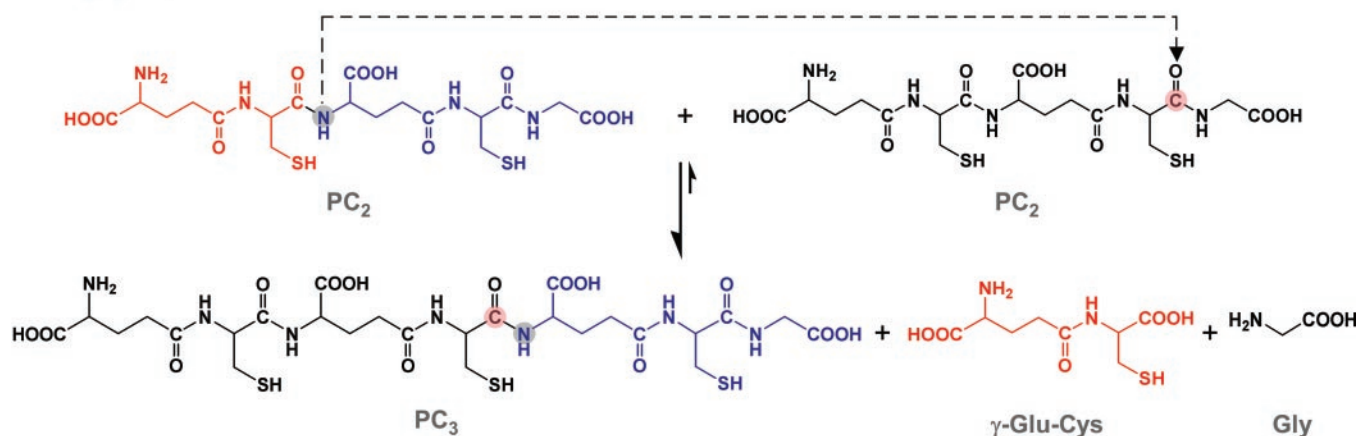
FIG. 1. PC synthase-catalyzed synthesis of PC 3 from PC 2 by dipeptidyl (A) or tripeptidyl (B) transfer. In dipeptidyl transfer (A), PC chain extension proceeds in the C- to N-terminal direction and is not associated with the production of des-Gly-PCs according to the general equation PC_n + PC_m \rightarrow PC_{n+1} + PC_{m-1} , where PC_1 = \text{GSH} . In tripeptidyl transfer (B), PC chain extension proceeds in the N- to C-terminal direction and is associated with the production of des-Gly-PCs according to the general equation PC_n + PC_m \rightarrow PC_{n+1} + \text{des-Gly-PC}_{m-1} + \text{G} , where \text{des-Gly-PC}_1 = \gamma\text{-Glu-Cys} .
