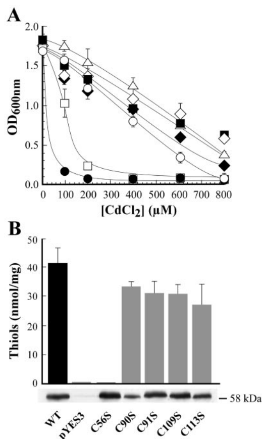
FIG. 9. Effect of heterologously expressed wild-type and Cys-to-Ser mutant-substituted AtPCS1-FLAG on the Cd 2+ hypersensitivity (A) and PC synthetic capacity (B) of mutant S. cerevisiae ycf1 \Delta strain DTY167. Strain DTY167 was transformed with the pYES3-AtPCS1-FLAG vector encoding wild-type (WT) AtPCS1 (○) or mutant AtPCS1 in which the Cys residue at position 56 (□), 90 (■), 91 (◇), 109 (◆), or 113 (△) had been substituted with Ser or with the empty pYES3 vector (●). To assess Cd 2+ hypersensitivity (A), the transformants were grown at 30 °C to A 600 ~ 1.8 in AHC medium supplemented with glucose and tryptophan before inoculating aliquots into 2-ml volumes of the same medium containing the indicated concentrations of CdCl 2 . A 600 was measured after growth for 24 h. To assess PC synthetic activity (B), the nonprotein thiols from the soluble fractions extracted from the same transformants after 24 h of growth in liquid medium containing CdCl 2 (50 \mu M) were fractionated by RP-HPLC and quantitated spectrophotometrically after reaction with DTNB. Values shown are means \pm S.E. ( n = 3-5 ). Also shown are the results of SDS-PAGE and Western analysis of wild-type and mutant AtPCS1-FLAG after heterologous expression. Aliquots (20 \mu g of protein) of the soluble fractions from the transformants were electrophoresed, electrotransferred to nitrocellulose membranes, and probed with anti-FLAG monoclonal antibody M2. The 58-kDa polypeptide was the only anti-FLAG antibody-immunoreactive band detected in the extracts.
