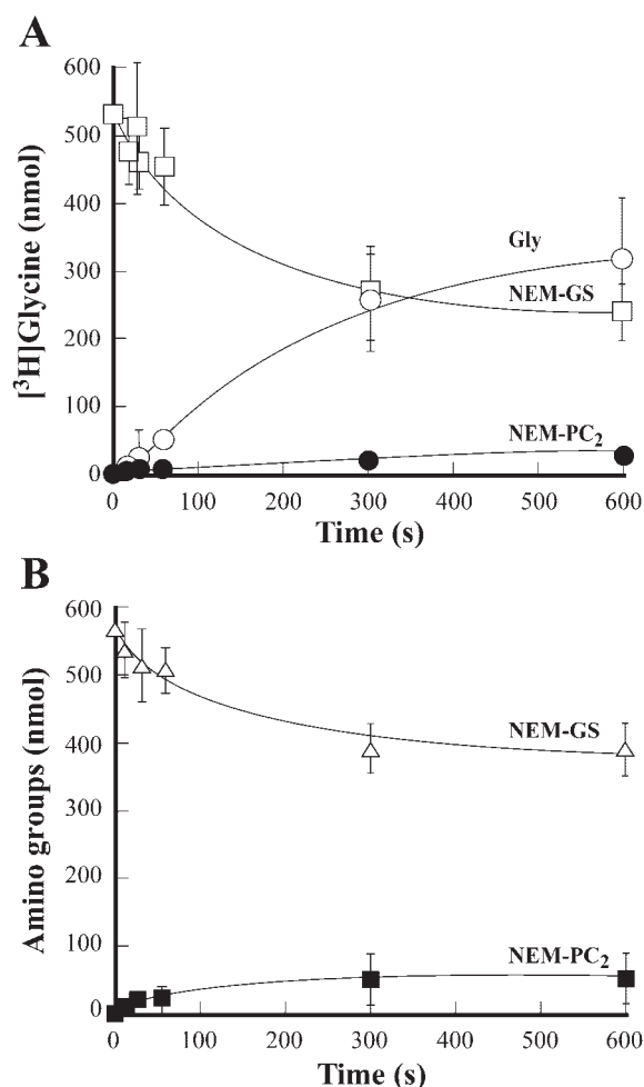
FIG. 8. AtPCS1-FLAG-catalyzed cleavage of glycine from NEM-GS. Aliquots of purified AtPCS1-FLAG (10 \mu g) were incubated with [ ^3 H]Gly-labeled NEM-GS (3 mM) in 100 mM HEPES/BTP buffer (pH 8.0) lacking CdCl 2 . At the times indicated, the reactions were terminated, and the amounts of free [ ^3 H]Gly generated (A) and the amounts of NEM-GS/NEM- \gamma -Glu-Cys and NEM-PC 2 (B) were estimated by liquid scintillation counting and the determination of N-terminal amino groups by reaction with fluorescamine, respectively, after RP-HPLC. Values shown are means \pm S.E. ( n = 3-5 ).
