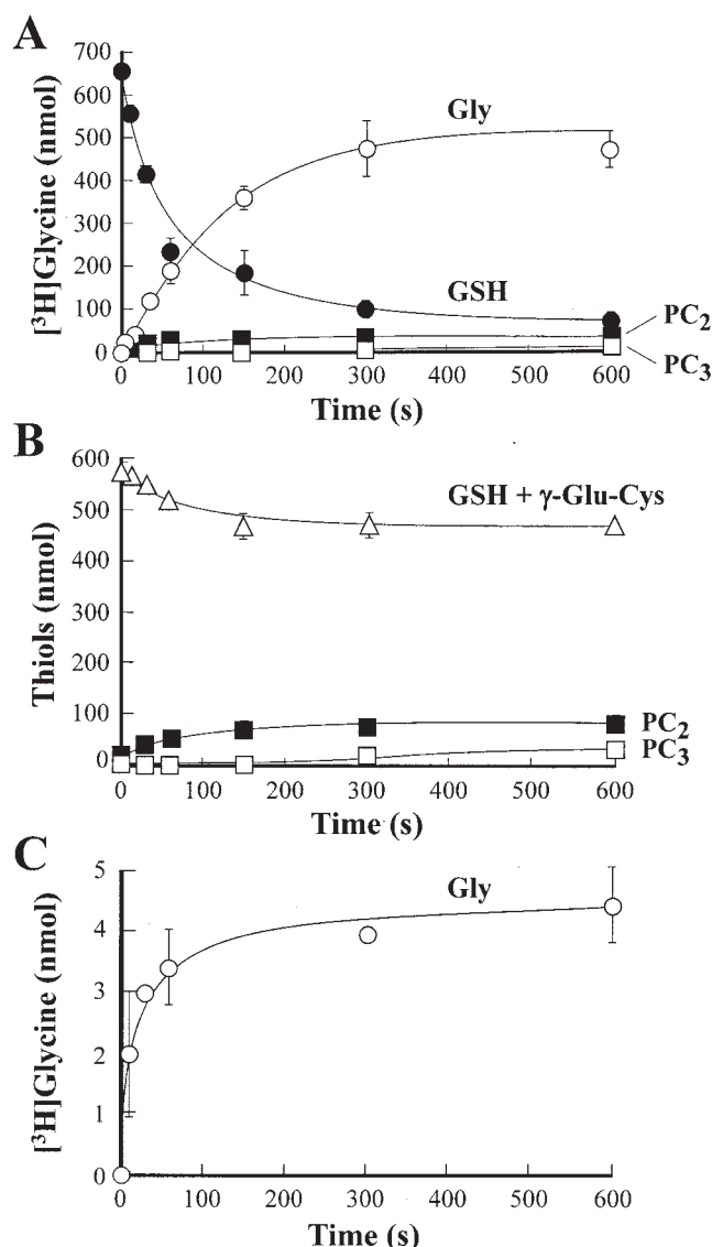
FIG. 6. AtPCS1-FLAG-catalyzed cleavage of glycine from GSH. Aliquots of purified AtPCS1-FLAG (10 \mu g) were incubated with [ ^3\text{H} ]Gly-labeled GSH (3 mM) in 100 mM HEPES/BTP buffer (pH 8.0) in the presence (A and B) or absence (C) of \text{CdCl}_2 (50 \mu M). At the times indicated, the reactions were terminated, and the amounts of free [ ^3\text{H} ]Gly generated (A and C) and the thiol contents of the GSH/ \gamma -Glu-Cys and \text{PC}_2 pools (B) were estimated by liquid scintillation counting and by reaction with DTNB, respectively, after RP-HPLC. Values shown are means \pm S.E. ( n = 3-5 ).
