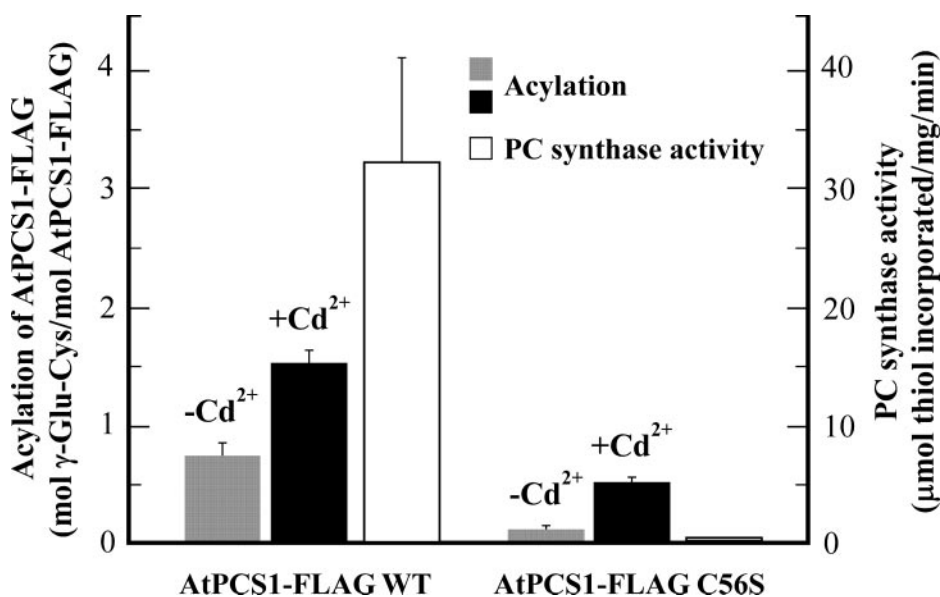
FIG. 11. In vitro PC synthetic activity and susceptibility of wild-type and C56S-substituted AtPCS1-FLAG to γ-Glu-Cys acylation. PC synthetic activity (□) was assayed by incubating immunoaffinity-purified wild-type AtPCS1-FLAG (WT; 1 μg/ml) or C56S-substituted AtPCS1-FLAG (1 μg/ml) with GSH (3.3 mM) and CdCl 2 (50 μM) at 30 °C for 10 min. Acylation of purified wild-type and C56S-substituted AtPCS1-FLAG by GSH in the absence (□) or presence (■) of Cd 2+ was assayed by incubation of enzyme (27.3 μg) with [ 35 S]Cys-labeled GSH (3 mM) in 100 mM HEPES/BTP buffer (pH 8.0) with or without CdCl 2 (50 μM) for 15 min before terminating the reaction and measuring enzyme acylation as described in the legend to Fig. 4.
