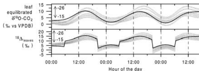
Fig. 10. Upper panel: \delta_{\text{leaf}} values equilibrated with \delta^{18}\text{O}\text{-H}_2\text{O} of leaf water calculated via Craig and Gordon with varying \varepsilon_{\text{kin}} from -26\text{‰} to -15\text{‰} . Lower panel: resulting variation in \Delta_{\text{leaves}} . Solid lines: standard simulation using measured bulk leaf water \delta^{18}\text{O} , symbols: test runs. Note that night-time values are not relevant to the model, as assimilation is set to zero.
