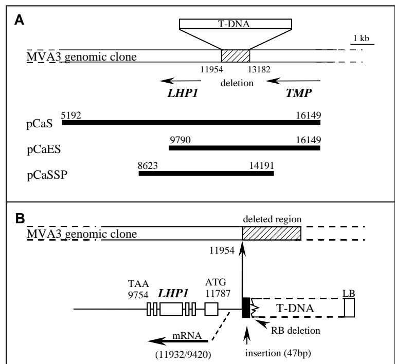
Fig. 2. Structure of the lhp1-1 locus. (A) Localisation of the 1.2 kb deletion on the genomic MVA3 P1 clone which accompanied the T-DNA region insertion in lhp1-1 . Database searches indicated two putative genes in this region, LHP1 and TMP . The plasmids, pCaS, pCaES and pCaSSP, were used for complementation experiments. (B) Detail of the T-DNA insertion in lhp1-1 . Insertion occurs at position 11954, 22 bp upstream of the 5' end of the isolated cDNA (11932). At the T-DNA right-border::genomic DNA junction, the integration was accompanied by deletions of the 24 bp RB repeat and the 21 bp adjacent to it. A small 47 bp insertion with no identified homology was also detected. The T-DNA LB was better conserved than the RB as commonly observed during T-DNA integration. Numbers refer to the sequence of the MVA3 P1 clone (accession number AB006706).
