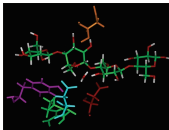
Fig. 10. View of the relative orientation of cellulotetraose and several important amino acid side chains for a final dynamics snapshot of a hydrated MD simulation conducted on the lowest energy structure found by pulling the P1 and P2 lobes together. The side chains shown are Asp117 (red), Asp265 (orange), Tyr73 (purple), Arg78 (green) and Asp79 (blue). A water molecule is also shown, hydrogen bonded to Asp79 and the O3 hydroxyl group of the sugar ring in the +1 binding site. Note that this water molecule is positioned below the aliphatic proton of the anomeric carbon of the sugar in the -1 site. If the scissile bond had actually been cleaved in this simulation, this carbon would be an achiral carbocation and this water molecule would be ideally positioned to donate a hydroxyl group to invert the stereochemistry, as is observed in E2. In this model, then, Asp79 would serve as the catalytic base.
