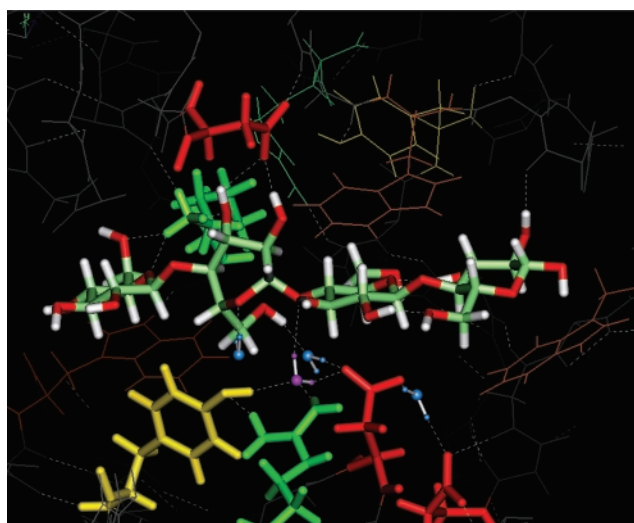
Fig. 4. Another view of the substrate in the binding cleft after 50 ps of simulation with the unprotonated Asp117 residue, indicating the relationship of the -1 sugar ring to various active site residues. Tyr73 is shown in yellow and Asp117 is shown in red below the oligosaccharides while Asp265 is shown in red above the substrate. Lys259 is shown in green behind the chain; steric crowding by this residue is responsible for tilting the plane of the sugar in the -1 site out of the plane of the chain. Arg78 is shown in green and several water molecules are also included. Hydrogen bonds are indicated by dashed white lines.
