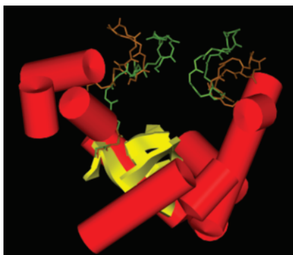
Fig. 8. A Richardson cartoon of E2, showing the secondary structural elements and indicating the initial positions of the two lobes P1 and P2 (see Figure 2) in orange and the lowest energy structure of these same loop chains in green, showing how the motion of the lobes has closed down the binding cleft into a tunnel such as is found in the exocellulase CBH II.
