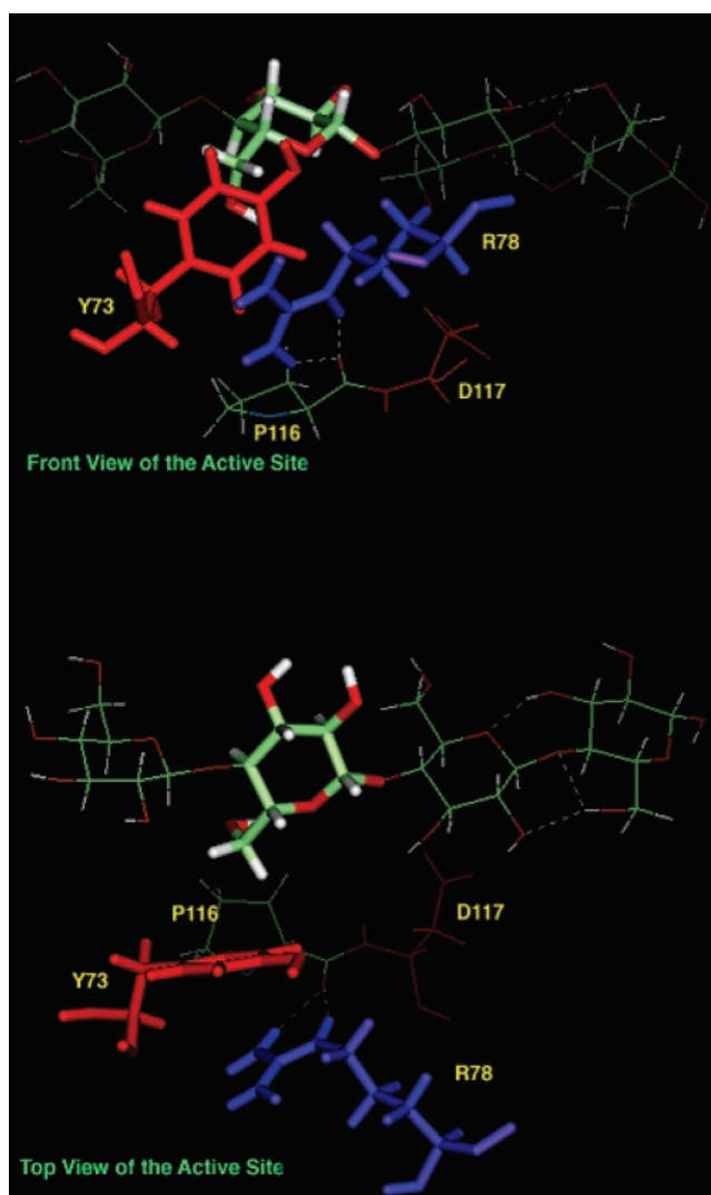
Fig. 1. Two views of the relative positions of the sugar ring in the -1 binding site, shown in thicker lines than the other three sugar rings, and Tyr73, Arg78, Pro116 and Asp117 in the minimized complex of the substrate with the crystallographic protein structure. Asp117 is the catalytic acid group, which, as can be seen, is far from the scissile bond.
