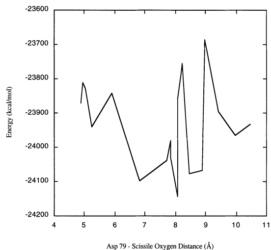
Fig. 7. Plot of the energy of the constrained E2–substrate complex as a function of the distance of the closest Asp79 oxygen atom to the glycosidic oxygen atom of the scissile bond. This distance is different from the constraint distance applied to the two lobes since the protein relaxes in a complex fashion at each value of the constraint distance, which is measured between the centers of mass of the two chains.
