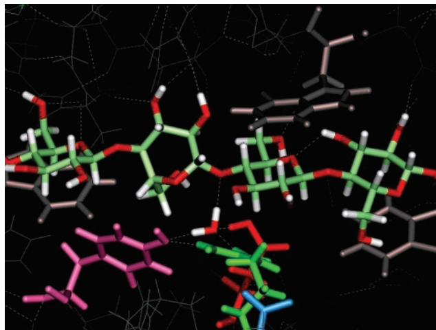
Fig. 5. Another view of the tetrasaccharide bound into the active site, in this case for the simulation in which Asp117, shown in red, is protonated, indicating how one water molecule bridges between this acid group and the glycosidic oxygen atom of the scissile bond. Also shown are Tyr73 in pink and Arg78 in green, with their hydrogen bonds to the same water molecule which serve to localize this molecule strongly in its bridging position. Asp79 is also shown in blue, far from the catalytic site, and Trp 41, 162 and 231, which stack against the hydrophobic faces of the sugar rings, are shown in gray.
