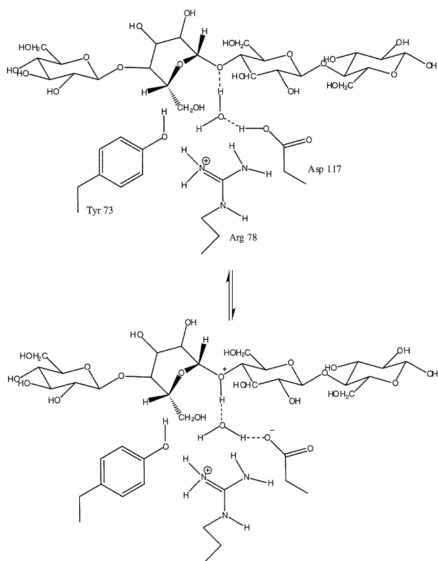
Fig. 9. Schematic representation of the proposed mechanism of E2 cellulase, showing cellulotetraose with the sugar in the -1 binding site distorted into a skew-boat. The Tyr73, Arg78 and Asp117 side chains are also indicated. In the proposed mechanism, following the shift in conformation of Arg78 and the ring flip in the substrate, a water molecule can comfortably hydrogen bond to the glycosidic oxygen atom, the catalytic acid group Asp117, the hydroxyl of Tyr73 and also to Arg78. This precise positioning allows a facile transfer of a proton from Asp117 to the water and from there to the glycosidic linkage. This step is then followed by the scission of the C1–O glycosidic bond of the sugar in the -1 site, producing an oxocarbenium ion and, in this example, a cellobiose leaving group. The ion would then be attacked by a hydroxyl group produced by the interaction of a water molecule with Asp79, which is positioned on the appropriate side of the binding cleft for this purpose (see Figure 10). The catalytic cycle would then be completed by the transfer of a proton from Asp79 to Asp117 via another bridging water molecule.
