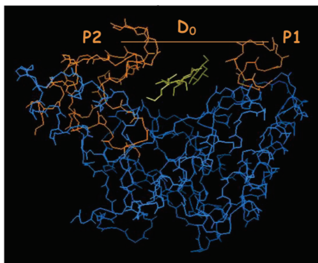
Fig. 2. Illustration of the positions of the two loops P1 and P2 in E2, as defined in the present simulations, and an indication of the constraint distance between their two centers of mass used to draw them together.
