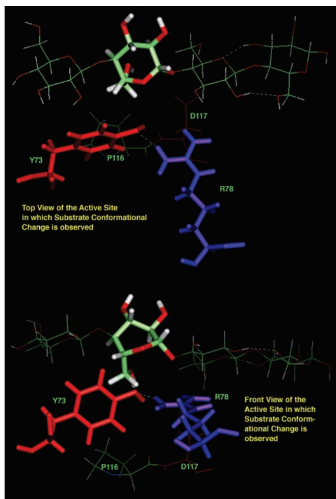
Fig. 3. Two views of the sugar ring in the -1 binding site after it has spontaneously ‘flipped’ during the course of a dynamics simulation into the {}^2S_0 conformation. Also shown are Tyr73 and Asp117.
