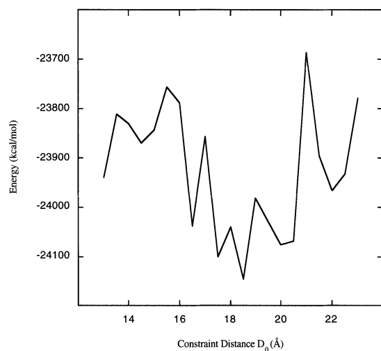
Fig. 6. Plot of the minimized energy of the E2–cellobiose substrate complex, constrained to move the P1 and P2 lobes to various relative separation distances d_0 , plotted as a function of d_0 . The constraint energy is not included in the total energy plotted.
