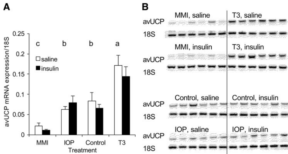
Fig. 4. A: avian uncoupling protein (avUCP) mRNA expression ( \pm SE) in gastrocnemius muscle of chickens at 26 days of age injected with either saline (open bars) or insulin (filled bars) solutions. B: RT-PCR products obtained from avUCP and 18S RNA. Products were stained using Vistra green (Amersham Pharmacia Biotech) and quantified with a Storm apparatus (Molecular Dynamics). Animals received control, MMI, T3, or IOP treatment. Different letters represent statistically different values between thyroid treatments in saline-treated chickens.
