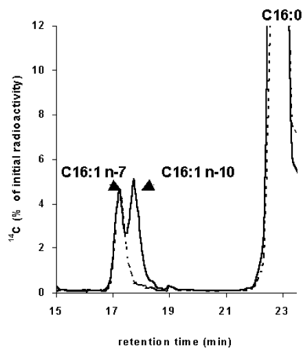
Fig. 3. HPLC analysis of cellular fatty acid naphthacyl esters from COS-7 cells incubated with [1-^{14}\text{C}] C16:0 and expressing rat \Delta 6 -desaturase versus control COS-7 cells. COS-7 cells transfected with pCMV/ \Delta 6 (large line) or nontransfected (dotted line) were cultivated for 24 h with albumin-bound [1-^{14}\text{C}] C16:0 (100 \mu\text{M} , 37 MBq/mmol). The identity of each fatty acid peak is indicated above the respective peak.
