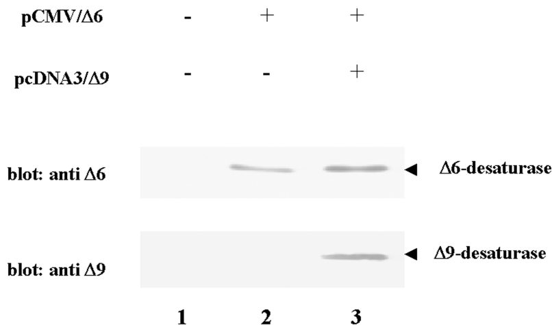
Fig. 1. Detection of rat \Delta 6 - and \Delta 9 -desaturases in transfected COS-7 cells by Western blot analysis. COS-7 cells were not transfected (lane 1), transfected with rat \Delta 6 -desaturase opening frame inserted in pCMV vector (pCMV/ \Delta 6 ) (lane 2) or transfected with both pCMV/ \Delta 6 and rat \Delta 9 -desaturase opening frame inserted in pcDNA3 vector (pcDNA3/ \Delta 9 ) (lane 3). COS-7 total cell homogenates (2 \mu g of protein) were resolved by SDS-PAGE and blotted. The blot was immunoprobed with anti-rat \Delta 6 -desaturase sera or anti-rat \Delta 9 -desaturase sera. Detection was performed using chemifluorescence (ECL Plus detection system).
