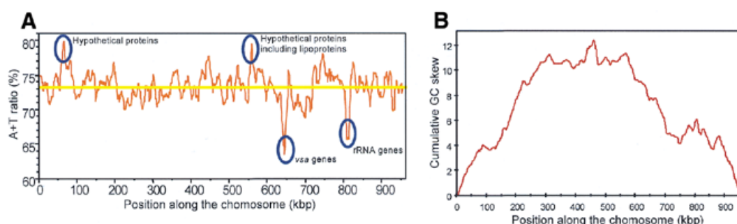
Figure 1. A + T ratio and cumulated GC skew along the M. pulmonis chromosome. (A) The curve indicates the A + T ratio along the M. pulmonis chromosome. This ratio was calculated with a sliding window of 10 kb with a step of 1 kb. The yellow line indicates the average A + T ratio for the genome. The identity of regions showing unusual A + T ratio is indicated. (B) The curve indicates the cumulated GC skew along the M. pulmonis chromosome starting at position 1 as defined in the text. The transition in GC skew is easily identified around position 1, the putative origin of replication of the chromosome. In contrast, the other transition which would correspond to the termination of replication is more difficult to identify because there are distinct peaks in the region centered around 460 kb.
