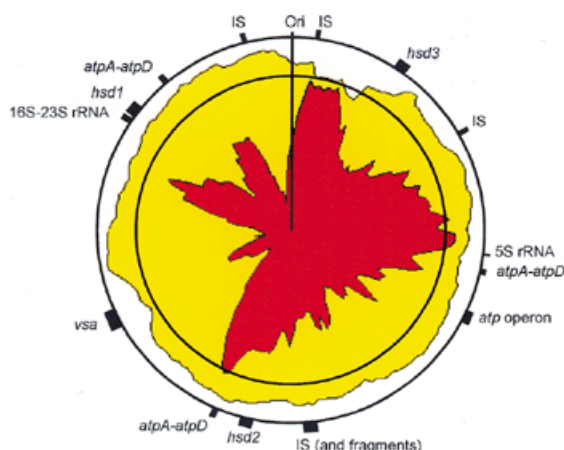
Figure 2. Density of coding sequences along the M. pulmonis chromosome. Yellow indicates the density of coding sequences in both strands of the sequence and red the density of the coding sequences in the clockwise strand (published sequence). This density was calculated with a sliding window of 50 kb. The first circle represents 100%, the second (inner circle) is 80%. The positions of rRNA genes and of other genes discussed in the text are indicated by black boxes.
