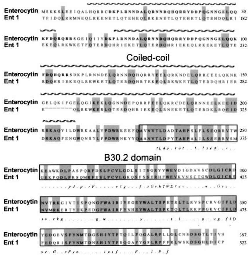
Fig. 5. A: Amino acid alignment of rabbit Enterocytin and guinea pig enterophilin 1 (Ent 1) (Gassama-Diagne et al., 2001). Sequences were aligned using the BLASTN and BLASTX network servers at NCBI. Light gray boxes indicate the existence of identical amino acid residues between the two proteins. Note that the first 132 amino acids of Ent 1 are not given here. The N-terminal sequence with a coiled-coil structure is represented by a spiral stretched length-wise. The two portions of Enterocytin sequence in the N-terminal domain shown in heavy type constitute two identical repeat units (from Asp18 to Ser 59 and from Asp 67 to Ser 108), apart from one residue underlined, by unity, in positions 55 and 104. The B30.2-like domain is
