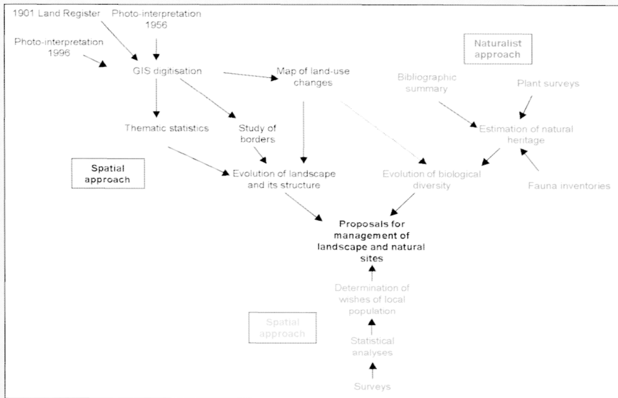
Diagram 1. General methodology.
