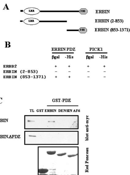
FIG. 4. Self-interaction of the ERBIN PDZ domain. A, schematic representation of full ERBIN (residues 1–1371), ERBIN (2–853) and ERBIN (853–1371). B, LexA-BD-ERBB2 and -ERBIN (2–853) and (853–1371) were transformed in L40 yeast with GAL4-AD-ERBIN PDZ domain or PICK1. Co-transformed yeast were plated on –Trp-Leu-His medium containing 10 mM 3-AT. + means growth on the selective medium (–His) and positive \beta -galactosidase activity ( \beta gal). C, Myc-tagged ERBIN wild type (ERBIN) or deleted of the PDZ domain (ERBIN. \Delta PDZ) expressed in COS cells were pulled down with GST, GST-ERBIN, -DENSIN-180, and -AF6 PDZ domains. Bound proteins were probed with anti-Myc antibody. One tenth of the lysate was run as total lysate (TL). Ponceau Red staining shows comparable amount of GST proteins.
