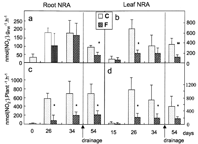
Figure 5. Nitrate Reductase Activity ( \text{nmol NO}_2^- \text{g}_{\text{FW}}^{-1} \text{h}^{-1} ) measured in fine roots (a) and in first flush leaves (b) of flooded (F) and control (C) Quercus robur seedlings harvested during flooding and 14 days after drainage (day 54). Results are also presented per plant organ (c, d) ( \text{nmol NO}_2^- \text{Plant organ}^{-1} \text{h}^{-1} ). Mean \pm SE, n = 5 , n = 3 in flooded root at days 0, 26 and 34, n = 4 in control roots at days 26 and 54. (*) and (**) indicate significant differences between flooded and control at p < 0.05 and p < 0.01 respectively; (Mann and Whitney test).
