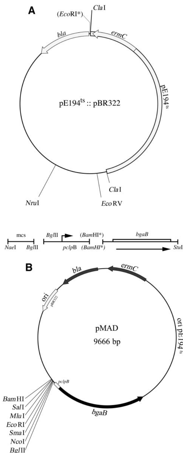
FIG. 1. Physical map of pE194 ts ::pBR322 and its derivative pMAD. (A) Construction of the pMAD plasmid. DNA fragments used to construct pMAD are indicated: mcs, multiple cloning site; pcpB , DNA fragment from S. aureus containing the clpB promoter region; bgaB , DNA fragment containing the promoterless bgaB gene encoding a thermostable \beta -galactosidase (8). Asterisks indicate restriction sites which have been lost during the construction steps. (B) Map of the pMAD plasmid. Unique restriction sites are indicated.
