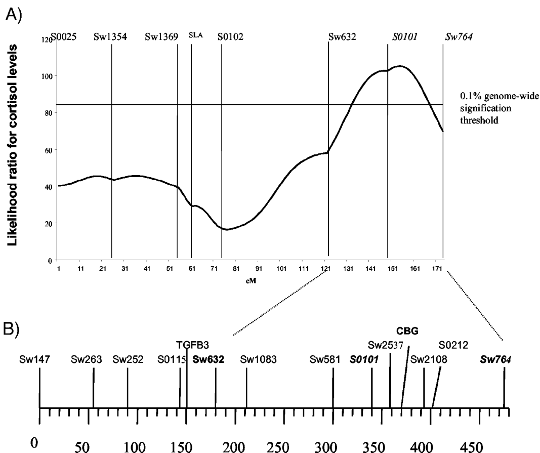
Fig. 1. Localization of Pig Cbg by Radiation Hybrids Mapping in the Cortisol Associated QTL Interval The QTL associated with cortisol levels (18) is shown in A (evolution of maximum likelihood ratio test along Sscr 7 for plasma cortisol concentrations). Detailed RH map of the QTL interval is shown in B (framework radiation hybrid map of swine chromosome 7 distances are in cR_{7000} ).
