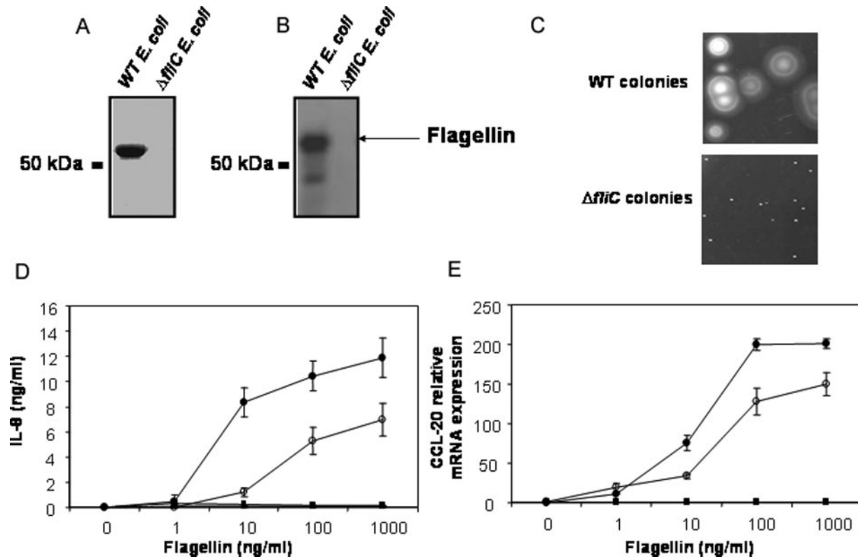
FIG. 2. Dose-dependent induction of IL-8 secretion and CCL-20 expression by concentrated E. coli flagellin. Concentrated WT and \Delta fliC E. coli -CM were analyzed after SDS/PAGE and Coomassie Blue staining (A) and by immunoblotting with an antiserum against Salmonella H7 flagellin (B). C, growth at 24 h on soft agar plates of WT and \Delta fliC E. coli colonies. D and E, HT29-19A (filled symbols) and Caco-2 (open symbols) IECs were stimulated either with flagellin concentrated from WT E. coli -CM (circles) at the indicated concentrations (1–1000 ng/ml) or with equivalent volumes of concentrated \Delta fliC E. coli -CM (squares). D, IL-8 secretion was assessed by ELISA after a 16-h stimulation. E, CCL-20 mRNA expression was analyzed by real-time quantitative PCR after a 6-h stimulation. Data are mean \pm S.E. for a triplicate experiment representative of at least three experiments (D and E).
