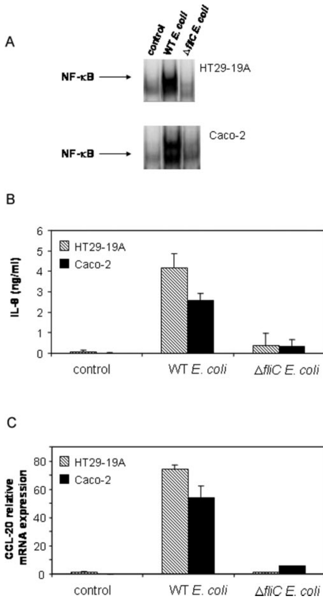
FIG. 3. Flagellin is the only factor responsible for the pro-inflammatory response of IECs to E. coli MG1655. IEC lines were stimulated with either WT E. coli , mutant aflagellated \Delta fliC E. coli , or medium alone (control) as described in Fig. 1. A, NF- \kappa B DNA-binding activity was assessed by EMSA after 3 h. B, IL-8 protein secretion was measured by ELISA in supernatants of HT29-19A (hatched bars) or Caco-2 (black bars) cells stimulated for 16 h. C, CCL-20 mRNA expression was measured by real-time quantitative PCR on RNA extracted from IECs after a 6-h stimulation. Data are mean \pm S.E. for a triplicate experiment representative of at least five experiments (B and C).
