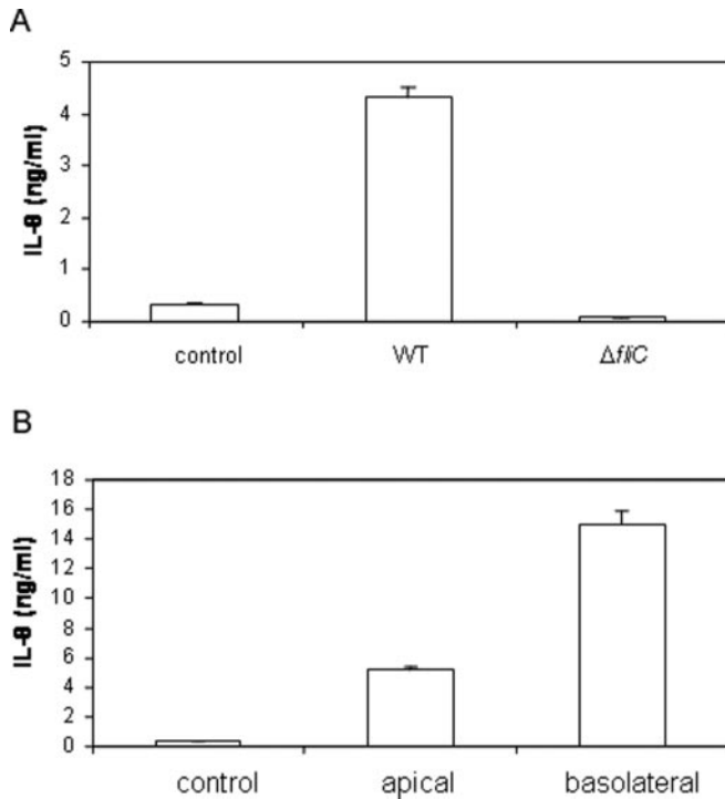
FIG. 5. Apical stimulation of polarized HT29-19A cells by live E. coli or flagellin induces basolateral secretion of IL-8. A, basolateral secretion of IL-8 in polarized HT29-19A cells stimulated on their apical side with either the WT E. coli , the \Delta fliC mutant (100 bacteria/cell), or medium alone ( control ) for 16 h. B, polarized HT29-19A cells were not stimulated ( control ) or stimulated with flagellin concentrated from WT E. coli -CM (100 ng/ml) added either to the apical or to the basolateral compartment. IL-8 secretion was assessed by ELISA in the basolateral supernatants. Data are mean \pm S.E. of triplicates in one experiment representative of at least three distinct experiments.
