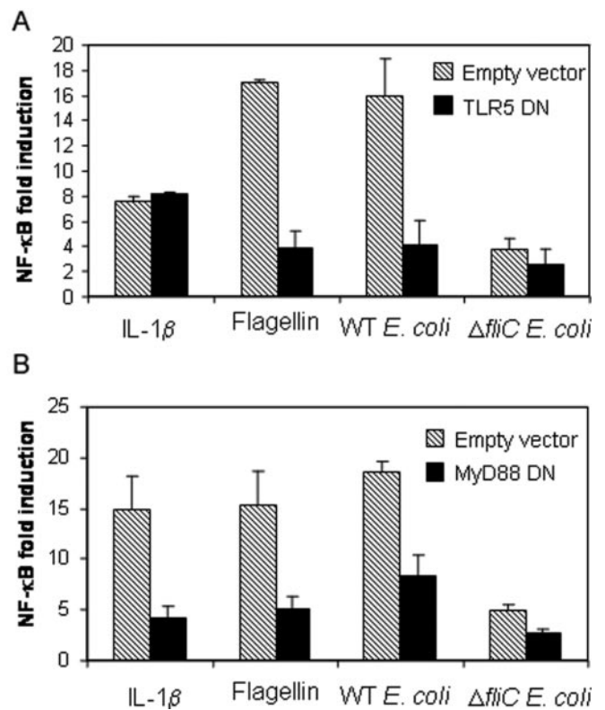
FIG. 4. Commensal E. coli -induced NF- \kappa B activity in IECs depends on the TLR5- and MyD88-signaling pathway. HT29-19A cells were transfected with NF- \kappa B Ig \kappa luciferase reporter alone (A and B, hatched bars) or in combination with either dominant negative TLR5 (A, black bars) or dominant negative MyD88 (B, black bars). Cells were then stimulated with either WT E. coli , mutant aflagellated \Delta fliC E. coli , IL-1 \beta as in Fig. 1, or flagellin concentrated from WT E. coli -CM (100 \mu g/ml) for 8 h. Luciferase activities were determined and normalized based on Renilla luciferase activity. Data are mean \pm S.E. of triplicates in one experiment representative of at least three distinct experiments.
