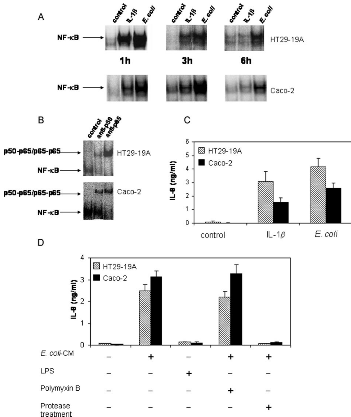
FIG. 1. E. coli induces NF-κB DNA-binding activity and IL-8 secretion by IECs via a soluble protein. A , time course of NF-κB DNA-binding activity was assessed by EMSA in HT29-19A and Caco-2 cell lines stimulated either with the commensal E. coli MG1655 strain (100 bacteria/cell), with IL-1β (10 ng/ml) or with medium alone (control), for 1–6 h. B , for supershift assays, nuclear extracts from HT29-19A and Caco-2 cell were stimulated with the commensal E. coli MG1655 strain for 3 h and NF-κB DNA-binding activity was tested by EMSA before (control) or after preincubation with antibodies against p50 or p65 NF-κB subunits. C , IL-8 protein secretion was measured by ELISA in supernatants of HT29-19A (hatched bars) or Caco-2 (black bars) cells stimulated for 16 h. D , HT29-19A (hatched bars) and Caco-2 (black bars) cells were cultured with either E. coli -conditioned medium (-CM) (1:6 dilution) with or without polymyxin B (10 μg/ml), LPS (1 μg/ml), or E. coli -CM after protease treatment. After 16 h of stimulation, IL-8 protein secretion was measured by ELISA in supernatants. Data are mean ± S.E. for a triplicate experiment representative of at least three ( D ) or five ( C ) experiments.
