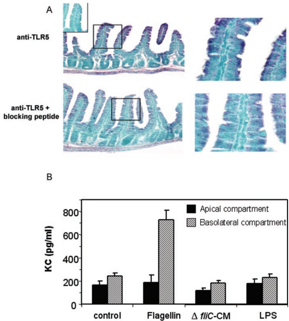
FIG. 6. Apical commensal E. coli flagellin induces basolateral secretion of KC by murine ileal biopsies. A , staining of enterocytes by anti-TLR5 antibody. Upper panel : ileal sections from C3H/HeN mice were stained with an anti-TLR5 goat antibody ( upper left panel , \times 100 ; upper right panel , \times 400 ). The inset in the upper left panel shows staining with a control polyclonal goat antibody. Lower panel : anti-TLR5 antibody was preincubated overnight with TLR5 blocking peptide prior to immunostaining ( lower left panel , \times 100 ; lower right panel , \times 400 ). B , KC secretion by intestinal biopsies. Murine ileal biopsies were mounted in Ussing chambers and stimulated apically with either flagellin concentrated from WT E. coli -CM (500 \mu\text{g/ml} ), concentrated \Delta fliC E. coli -CM (equivalent volume of concentrated WT E. coli -CM), LPS (100 \text{ng/ml} ), or medium alone ( control ). After a 4-h stimulation, KC secretion was measured by ELISA in both apical ( black bars ) and basolateral ( hatched bars ) compartments. Data are mean \pm S.E. of triplicates in one experiment representative of at least five distinct experiments.
