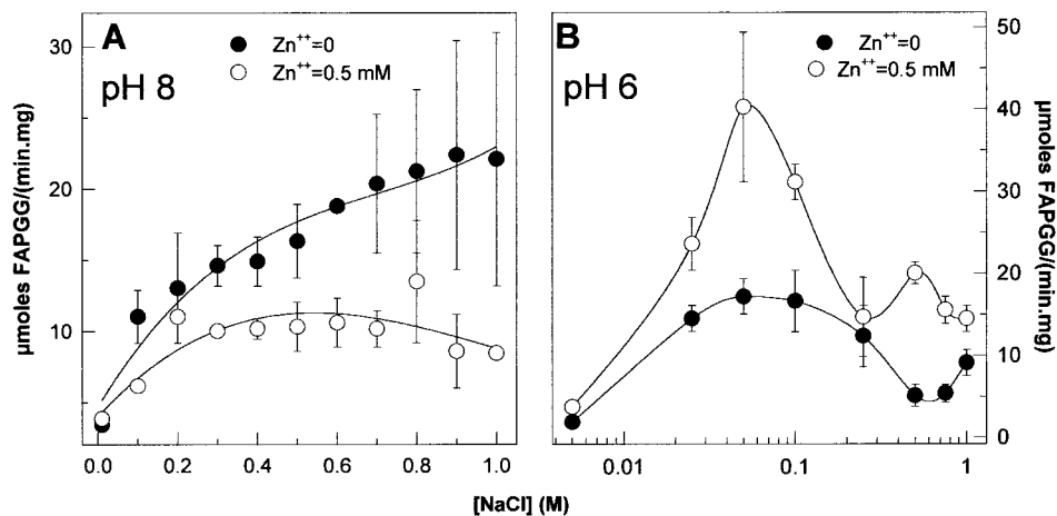
FIG. 3. Effect of \text{Cl}^- and zinc concentrations at pH 8 and pH 6. The FAPGG hydrolysis by the purified enzyme was measured at varying \text{Cl}^- concentrations in the absence (●) or presence (○) of 0.5 mM zinc at pH 8 (A) or pH 6 (B) (mean \pm SD for three experiments). Note that the scale is logarithmic for B.
