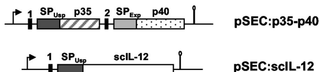
FIG. 2. Expression cassettes to produce and secrete IL-12 in L. lactis : schematic structures of p35 and p40 subunits and scIL-12 cassette expressed under the lactococcal P nisA promoter and carried by the plasmids indicated. For details concerning plasmid construction, see the text and Table 1. The arrows indicate the presence of the nisin-inducible promoter (P nisA ); the solid vertical bars indicate the RBS of the usp45 gene (bar 1 for p35) or of the exp4 gene (bar 2 for p40); the dark gray bars indicate the SP of the usp45 gene; the light gray bar indicates the SP of the exp4 gene (48); the cross-hatched bar indicates the p35 mature coding sequence; the dotted bar indicates the p40 mature coding sequence; the open bar indicates the scIL-12 coding sequence; and the stem-loop symbols indicate trpA transcription terminators (not to scale).
