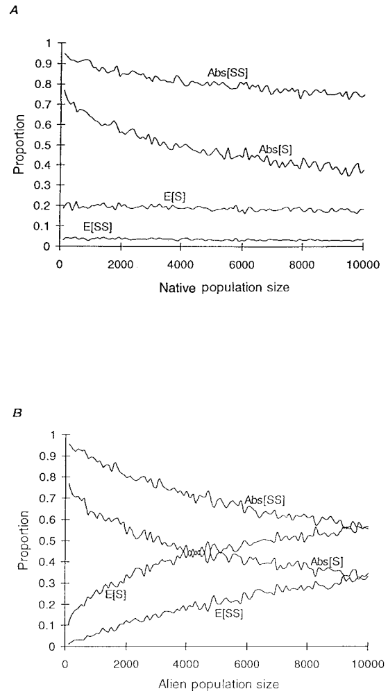
FIG. 2.—Relationship between the population size of the alien ( N_a ) and native ( N_n ) populations and E[SS] and S or Abs[SS] and S statistics. N_n or N_a values vary by steps of 100 from 100 to 10,000 with values of N_a (A) and N_n (B) kept constant at 500. The divergence time was kept at 50,000 generations. Other marker parameters are as in the standard simulation conditions.
