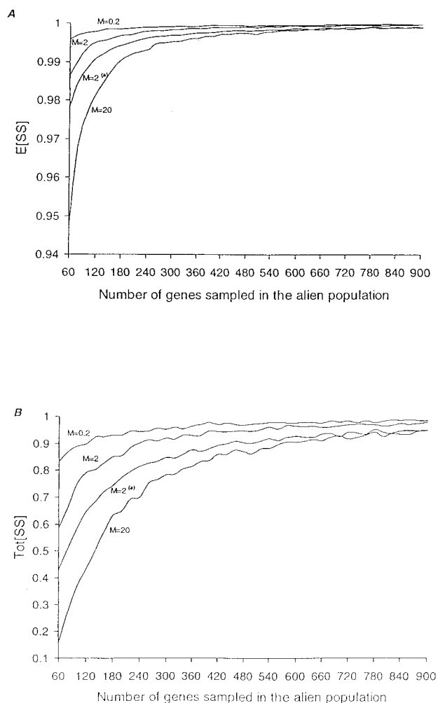
FIG. 5.—Effect of the number of genes sampled in the alien population on (A) E[SS] and (B) Tot[SS] statistics for different M = 4N\mu values and assuming an SMM or a TPM (a) with P = 0.674 and \alpha = 0.5 . The divergence time was kept constant at zero generations.
