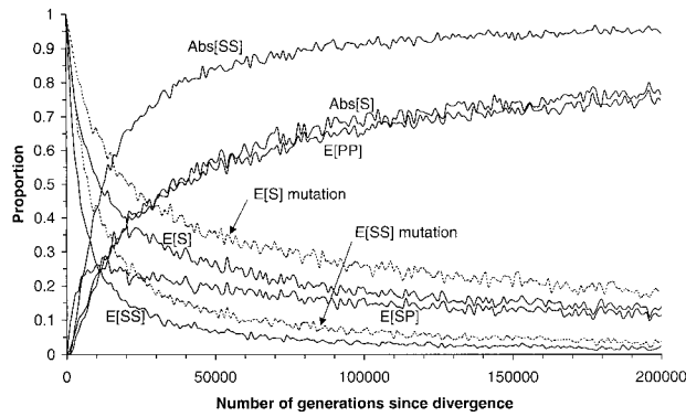
FIG. 1.—Relationship between the divergence time and E[SS] , SP , and PP or Abs[SS] , SP , and PP statistics for a JMS, as well as for a single-site microsatellite locus ( E[S] and Abs[S] ). Population and marker parameters correspond to standard simulation conditions, i.e., N = 1,000 for both populations and \mu = 5 \times 10^{-4} for both microsatellite sites, with the latter following an SMM with no allele size constraint. The dashed curves represent the contribution of mutations to the decline of E[SS] and E[S] with time (see text for details).
