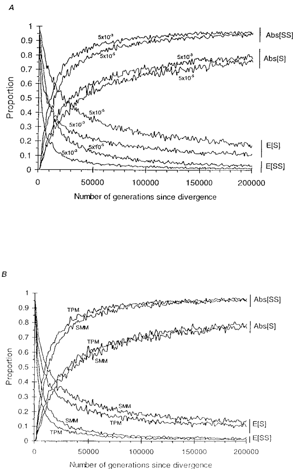
FIG. 3.—Effect of the mutation rate ( \mu = 5 \times 10^{-5} and 5 \times 10^{-3} ) on E[SS] and S and Abs[SS] and S statistics (A) and effect of large mutation steps (B). TPM parameters are P = 0.674 and \alpha = 0.5 . Other population and marker parameters are as in the standard simulation conditions.
