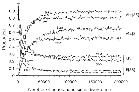
FIG. 4.—Effect of allele size constraints ( R = 20 and 50 ) on E[SS] and S and Abs[SS] and S statistics (fig. 4A). Effect of the mutation model assuming allele size constraint with R = 20 (fig. 4B). TPM parameters are P = 0.674 and \alpha = 0.5 . Other population and marker parameters are as in the standard simulation conditions.
