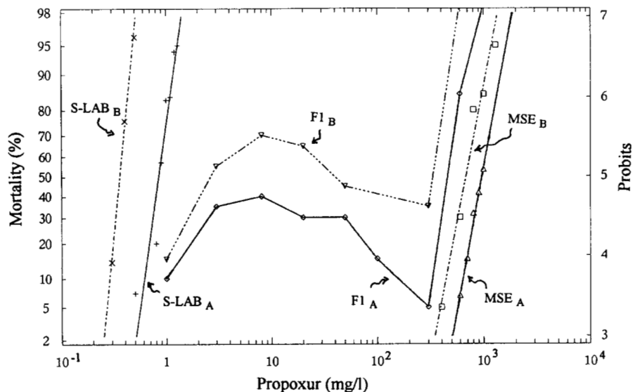
FIGURE 5.—Effect of the type of cup (Ca vs. Cb) in bioassays of the susceptible strain (S-LAB), the resistant strain (MSE) and the F 1 with propoxur in the B environment (with Fc and Wc). ---, cup Cb; —, cup Ca. See text for explanations.
