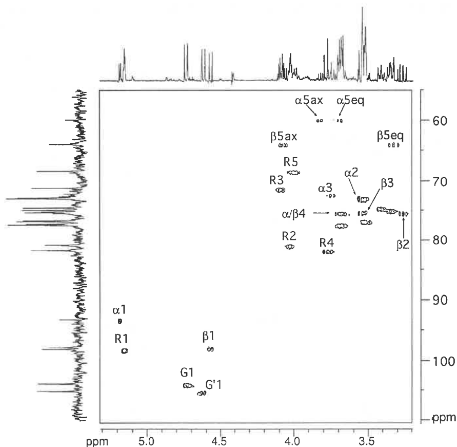
Fig. 6. 2D ^1\text{H} - ^{13}\text{C} chemical shift correlation spectroscopy (HMQC) contour plot obtained for oligosaccharide D3 at 55 ^\circ\text{C} . Letters R, G, G', \alpha and \beta refer to Rha, GlcA linked to O-4 of Rha, GlcA linked to O-2 of Rha, Xyl \alpha and Xyl \beta , respectively; numbers correspond to the proton/carbon in the residues; ax and eq refer to axial and equatorial, respectively. High resolution 1D ^1\text{H} and ^{13}\text{C} spectra are represented along the F2 and F1 axes, respectively.
