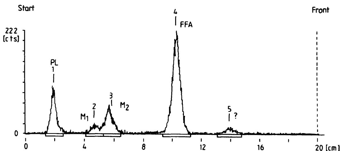
Fig. 3. Radiochromatogram obtained after elution of lipids extracted from rat platelets after 4 min of incubation in the presence of arachidonic acid (7.5 \mu\text{M} ) and radiolabeled 20:4 \Delta 14t (7.5 \mu\text{M} ). The mobile phase was hexane-diethyl ether-acetic acid 60:40:1 (v/v/v).
