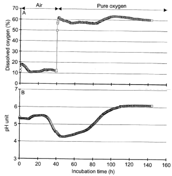
16 Fig. 3A,B Dissolved O (A) and pH (B) variations in the bubble-column reactor as a function of culture age
