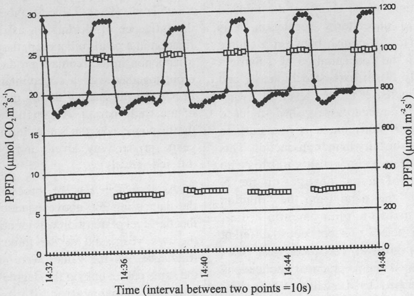
Fig. 9. Net \text{CO}_2 assimilation ( P_n ) of leaves of Digitaria decumbens grown under shade (33% sunlight) exposed alternately to low and high (sunflecks) levels of PPFD (—) (from Dulormne, 1997).
