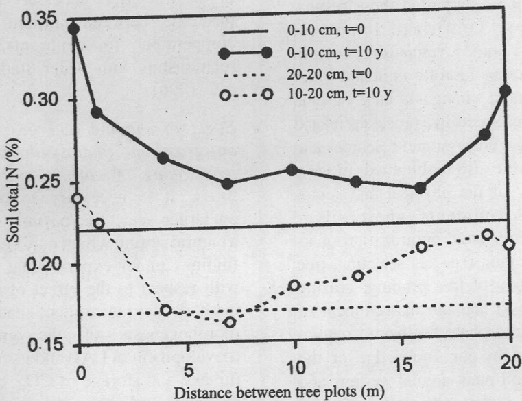
Fig. 10. Concentration of soil nitrogen in a grass plot ( Dichanthium spp. ) placed between two silvopastoral plots ( Gliricidia sepium , NFT). The tree rows correspond to distances 0 and 20 m; t = 0 and t = 10 y correspond to nitrogen concentration at the time of tree planting and 10 y afterwards, respectively (adapted from Dulormne et al. , 1999); soil depth sampled: 0-10 cm, 10-20 cm.
