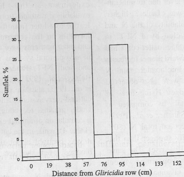
Fig. 8. Spatial distribution of sunflecks between two rows of Gliricidia sepium . Distance between rows = 3 m, IAF = 1.7 (from Dulormne, 1997). Sunflek = irradiance \geq 800 \mu\text{mol m}^{-2} \text{s}^{-1} for >0.6 s.
