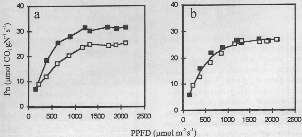
Fig. 5. Light response curves for net \text{CO}_2 assimilation ( P_n ) over a range of photosynthetic photon flux densities (PPFD) for leaves of Dichanthium aristatum grown in open (full sun □) or shade (■) expressed on (a) leaf area basis or on (b) leaf N amount basis (from Cruz, 1997a).
