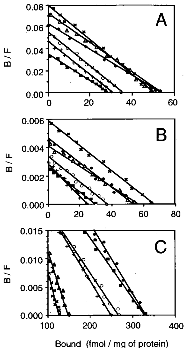
Figure 3 Scatchard plots of adrenoceptor saturation binding data for the 'Control group' and all 'TNBS-treated' groups. The ratio of bound to free (B/F) is expressed as a function of bound [ ^3 H]prazosin ( \alpha_1 -adrenoceptors; A), [ ^3 H]rauwolscine ( \alpha_2 -adrenoceptors; B) and [ ^3 H]DHA ( \beta -adrenoceptors; C). Each plot is representative of at least three determinations performed in duplicate [see Methods section for definition of experimental groups]. \square Control, \times TNBS, \triangle TNBS-INDO, \blacklozenge TNBS-MK, + TNBS-NAME, \circ TNBS-DOX.
