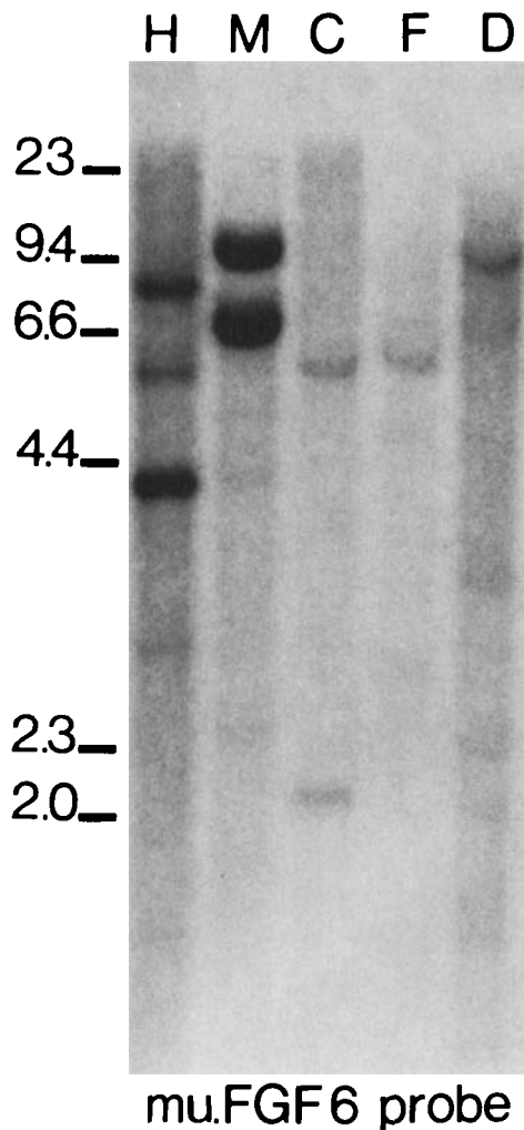
FIGURE 4. Conservation of the FGF6 gene. Southern "zoo blot" hybridization was carried out at 42°C, in 35% formamide, 5 \times SSC, 5 \times Denhardt's, on 10 \mu g of DNA from various species as follows: H, human; M, mouse; C, chicken; F, frog ( Xenopus laevis ); D, fly ( Drosophila melanogaster ). The probe used (probe PN) was a murine Fgf6 cDNA spanning the three coding exons.
