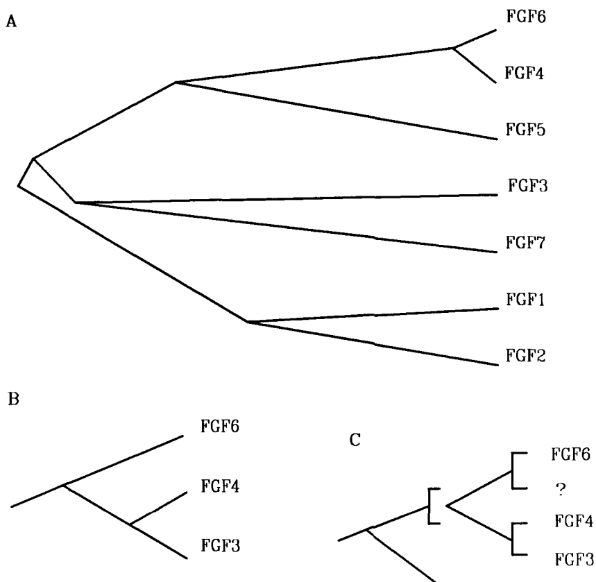
FIGURE 5. Phylogenetic FGF protein trees. A: Unrooted phylogenetic tree inferred from the amino acid sequences of the FGFs. The operational units (OU) present at the external nodes are the seven FGF proteins with names used in FIGURE 2. The tree shows one topology only (out of 954 theoretically possible given 7 OU; Reference 11). Branches are scaled, i.e., their lengths are proportional to the number of substitutions. B and C: portions of unrooted trees inferred from sequence and chromosomal localization data, with focus on three OU; FGF3 and FGF4 are clustered on chromosomal band 11q13, 13 while FGF6 lies on band 12pter. 10 In these particular trees, a specific rapid divergence of FGF3 ( B ) or a cluster duplication ( C ) is hypothesized.
