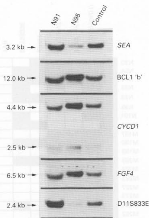
Figure 4 Amplification of D11S833E in the absence of an amplified BCL1-CYCD1-FGF3-FGF4 area. The experiment was performed as described in the legend to Figure 2. The SEA proto-oncogene, which is seldom amplified in breast tumors (Theillet et al. , 1990), indicates the basal ploidy of chromosome 11 sequences in each sample. DNA from tumor N95 served as a control for amplified 11q13 loci and was thus underloaded. Densitometric scanning of this autoradiogram indicated that D11S833E was amplified threefold in tumor N91
