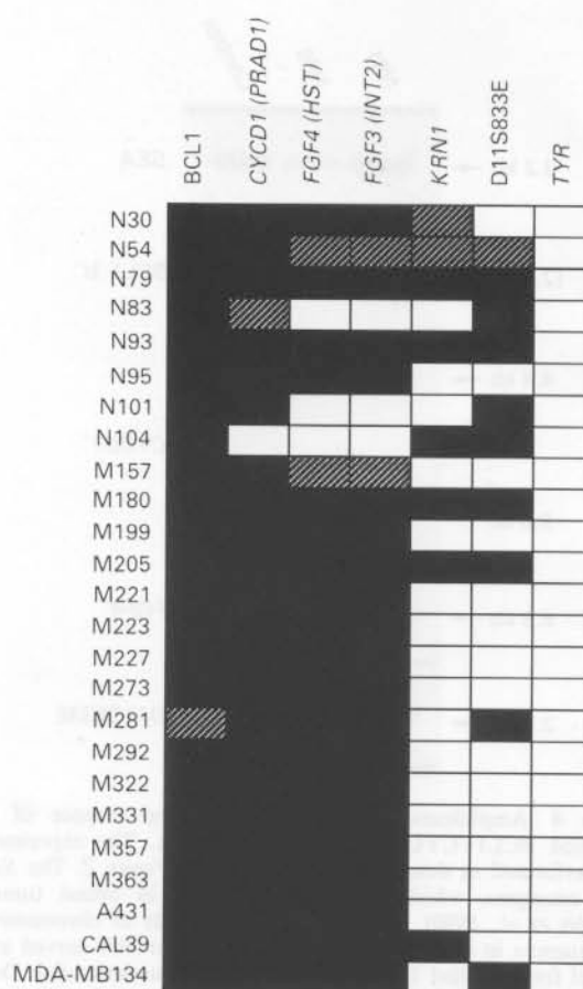
Figure 3 Discontinuities in a population of DNA samples bearing an amplification of BCL1. EcoRI-digested DNAs of 22 primary breast cancers and three cell lines, all amplified for BCL1, were analysed according to Figure 2. In order to avoid blot-to-blot variability, the same Southern blots were successively hybridized with every probe indicated. A black rectangle indicates that the marker was amplified at the highest level observed for amplification at 11q13 in the given sample, a white one that it was not amplified at all and a hatched one that it was definitively amplified but that other 11q13 markers have been found amplified at higher level (see, for example, D11S97 vs. BCL1 amplification of A431, in Figure 2).
