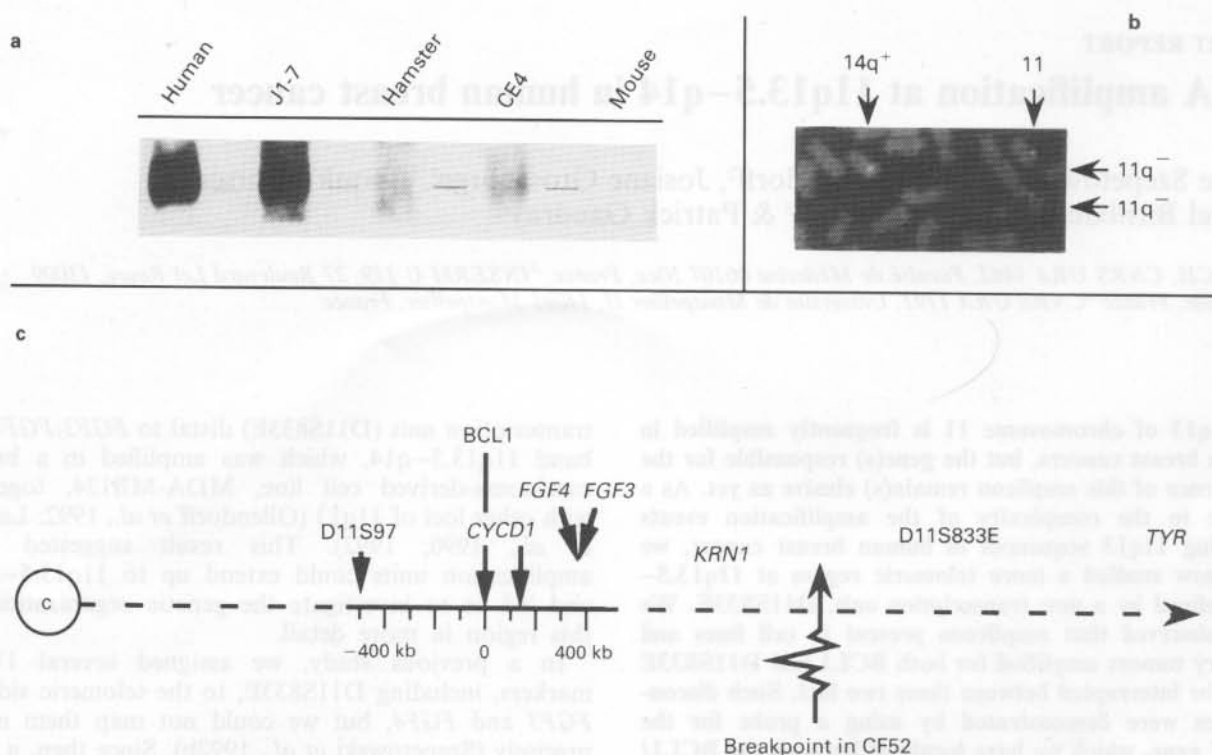
Figure 1 KRNI is located between FGF3 and D11S833E . (a) DNA isolated from normal human leukocytes, hybrid cell lines and their normal counterparts, hamster corresponding to J1-7 and mouse to CE4, was digested by Hind III restriction enzyme and analysed according to Szepietowski et al. (1992b). The KRNI probe used was the polymerase chain reaction (PCR) fragment highly specific for the bona fide KRNI gene located on 11q13 (Richard et al. , 1991). (b) Fluorescent in situ hybridization on Rec-1 cell line chromosomes was performed according to Szepietowski et al. (1992b). Normal 11, der14q + and two der11q - chromosomes are indicated by arrows. The probe was KRNI cDNA-containing plasmid. Therefore, the KRNI -like sequence known to be situated on 11p15 (MacKinnon et al. , 1991) is detected on the normal chromosome 11 as well as on the der11q - . (c) Physical map of 11q13 derived in part from a and b ( BCL1 represents the breakpoint in the CE4 somatic hybrid). The mapping of the breakpoint in the CF52 hybrid relies on both MacKinnon et al. (1991) for the absence of KRNI and Szepietowski et al. (1992b) for the presence of D11S833E in this cell line. Distances between BCL1 , CYCD1 and FGF3/FGF4 were reported in Lammie & Peters (1991)
