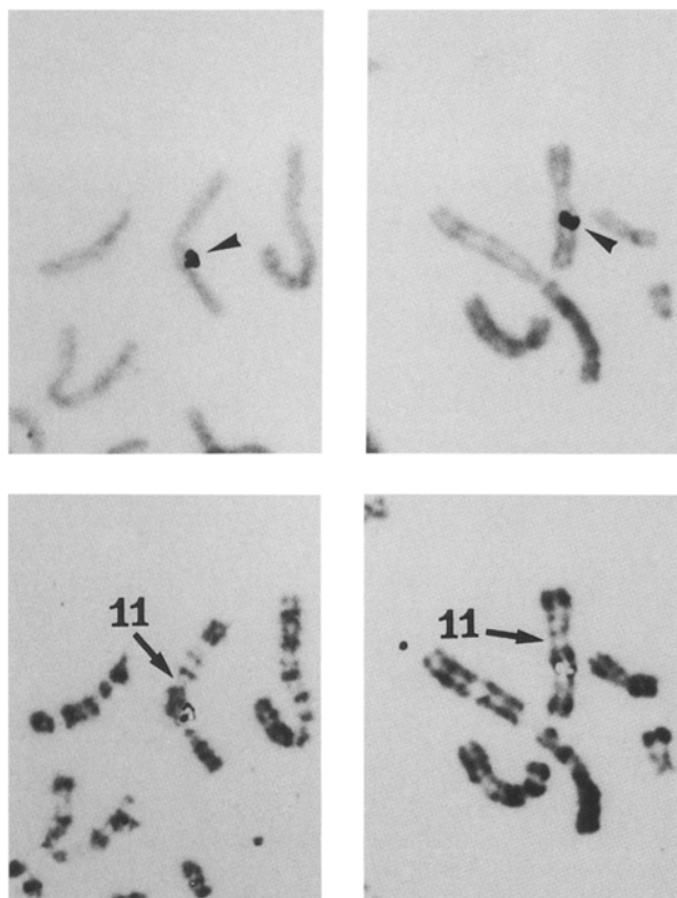
Fig. 1. Localization of cos 9 derived sequences (pDB 98) to human Chr 11, region q13.5-q14. (A) Two partial human metaphases showing the specific site of hybridization to Chr 11. Top: arrowheads indicate silver grains on Giemsa-stained chromosomes, after auto-
