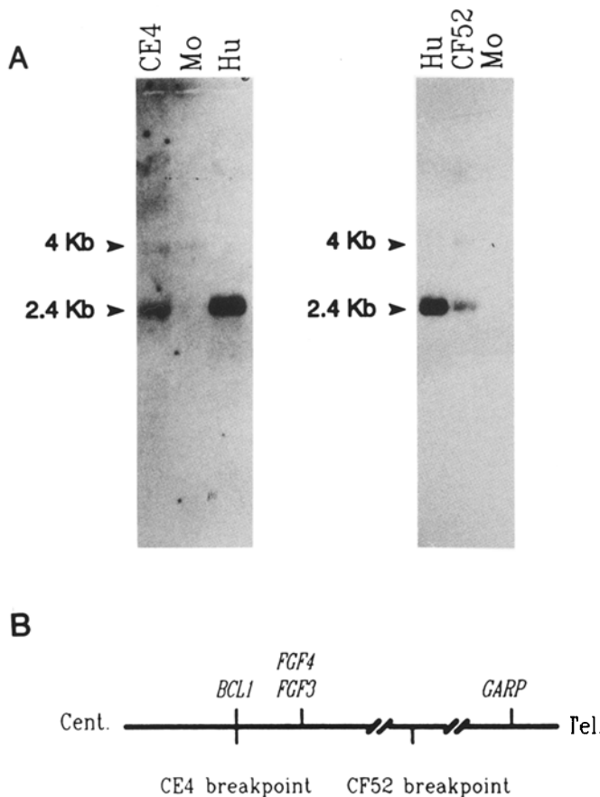
Fig. 2. On 11q, D11S833E ( GARP ) maps telomeric to BCL1 and FGF3/FGF4 . (A) Ten \mu g of mouse (lanes Mo), human (lanes Hu) and hybrid cell lines (lanes CE4 and CF52) DNAs were digested by EcoR I and run on agarose gels. Southern blot hybridizations with the human PR 98 probe shows bands of 2.4 kb in human and hybrids DNAs. Longer exposures of the blots detected a cross-reacting band of 4 kb in mouse and hybrids DNAs. (B) Diagram of human chromosome 11q13–q14 region showing the order of loci and breakpoints described in text.
