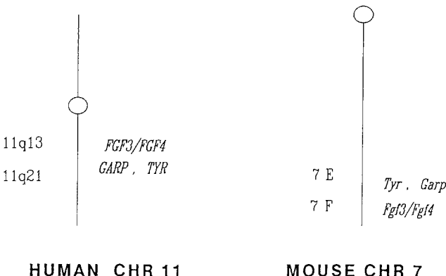
Fig. 5. Schematic representation of the human and mouse homologous regions containing GARP . Other loci of the conserved group of synteny are the TYR gene, located in human 11q14–q21 and mouse 7E, and the tandem of FGF genes, FGF3/INT2 and FGF4/HST , located in human 11q13.3 and mouse 7F. The precise location of GARP with respect to these loci is unknown. However, due to the data obtained from the chromosomal in situ hybridization experiments, it may be that GARP is located in between the FGF and TYR genes.
