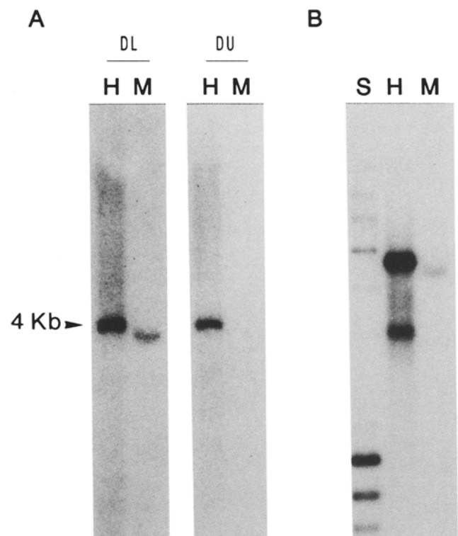
Fig. 3. Presence of a gene in the region defined by D11S833E. (A) Southern blot hybridization of human and murine DNAs with human probes derived from pDB98. Two DNA fragments, DL and DU, were used as probes to hybridize human (lanes H) and mouse (lanes M) DNAs, lighting up a 4 kb band in human (DL and DU) and in mouse (DL only). (B) Northern blot hybridization of human and murine RNA with a human GARP probe. The human StuI DNA fragment (see Material and methods) was used to hybridize human (lane H) and mouse (lane M) poly(A) + RNAs. Ten \mu g were loaded in each lane. Two human transcripts of 4.5 and 2.8 kb are detected in human and one of 4.3 kb in mouse, as determined using Ava I + Nar I fragments of phage \lambda and Hae III fragments of phage \phi X as size markers loaded in lane S.
