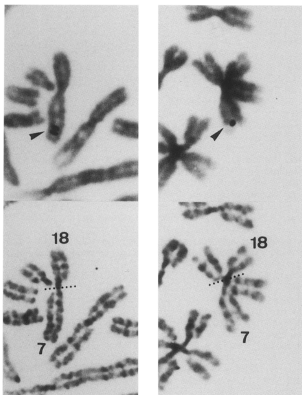
Fig. 4. Localization of the Garp gene to mouse Chr 7. (A) Two partial WMP mouse metaphases, showing the specific site of hybridization to Chr 7. Top: arrowheads indicate silver grains on Giemsa-stained chromosomes, after autoradiography. Bottom: chromosomes with silver grains were subsequently identified by R-banding. (B) Diagram of WMP mouse Rb(7;18) chromosome, indicating the distribution of labeled sites.
