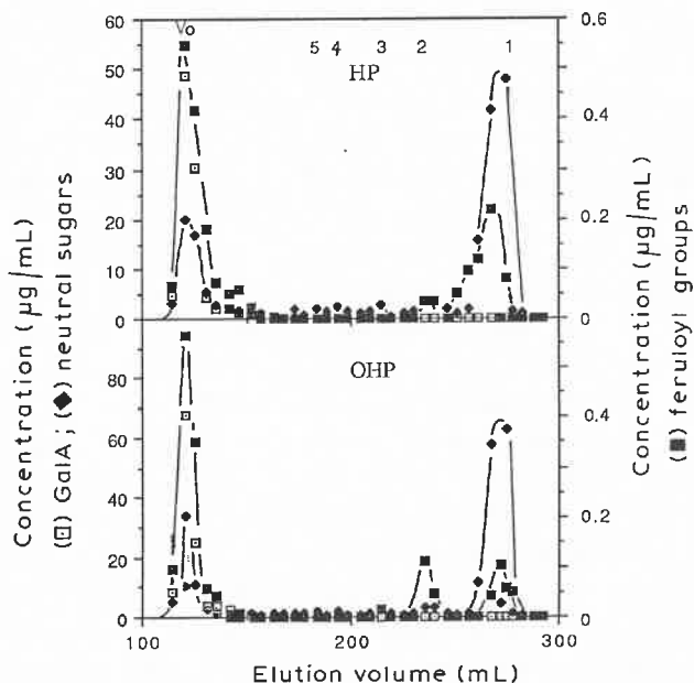
Fig. 5. Chromatography on Bio-Gel P-2 of HP and OHP "hairy" fragments degraded by 0.05M trifluoroacetic acid (100°, 1 h) after hydrolysis by Araf-ase (for 24 h).
