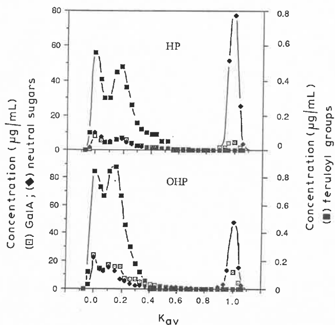
Fig. 4. Chromatography on Sephacryl S-200 of the products released from HP and OHP "hairy" fragments by hydrolysis with Araf-ase, endo-Ara-ase, and endo-Gal-ase in combination.
