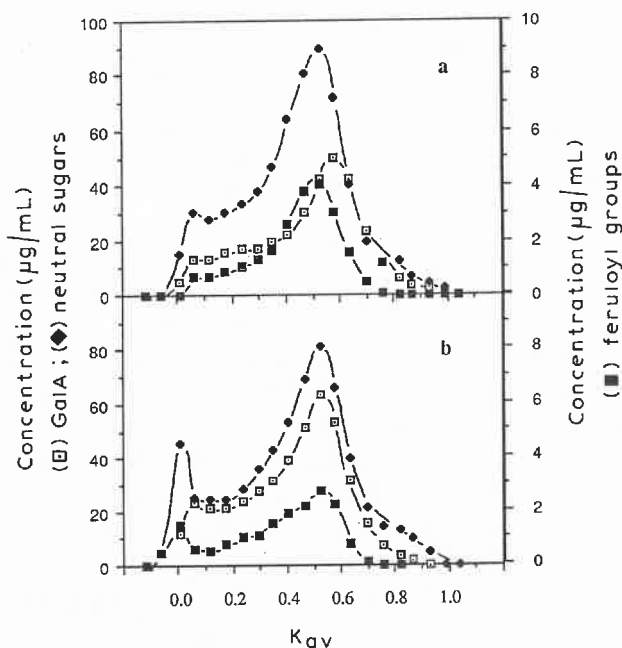
Fig. 3. Chromatography on Sepharose CL-6B of (a) retentate from HP "hairy" fragments degraded successively by Araf-ase (1.5 h), endo-Ara-ase, and endo-Gal-ase, (b) retentate from OHP "hairy" fragments as in (a).
