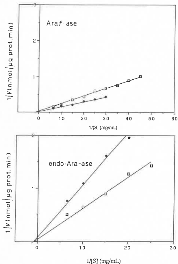
Fig. 2. Lineweaver-Burk plots of Araf-ase and endo-Ara-ase on "hairy" fragments of sugar-beet pectins: —□—, HP; —●—, OHP.
