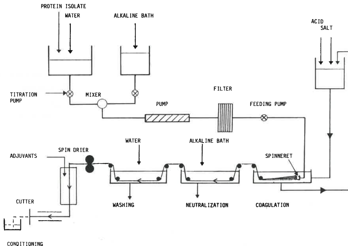
Fig. 1. Spun protein processing diagram (Culioli, 1981).
