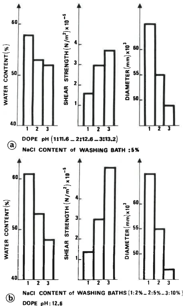
Fig. 4. Physical measurements on spun fababean protein fibres: a) evaluation of fibre bundle water content, shear strength and fibre diameter as a function of the dope pH (NaCl content of washing bath: 5%) and b) evaluation of fibre bundle water content, shear strength and fibre diameter as a function of bath NaCl content (dope pH:12.6).
