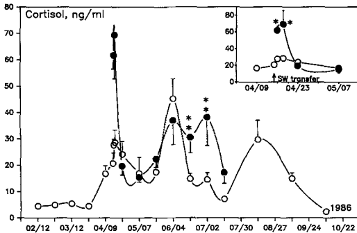
FIG. 1. Changes in plasma cortisol levels (mean and SEM) during the parr-smolt transformation of coho salmon maintained in fresh water (open circles) and during seawater adaptation (closed circles). Insert: Details of changes in plasma cortisol levels 1, 3, 7, and 14 days after seawater exposure. Asterisks denote significant differences ( * P < 0.01 ; ** P < 0.05 ) in levels between freshwater and seawater fish. n = 8-10 for each point. Absence of standard error bars indicates that the SEM was smaller than the symbol.
