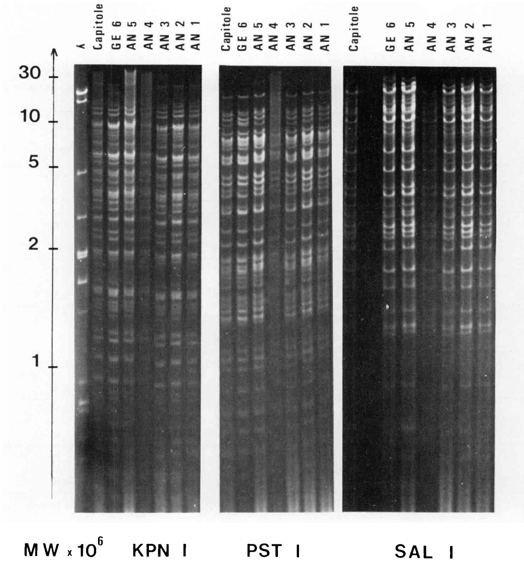
Figure 1 Electrophoregrams of restriction fragments obtained after cleavage with the KPN I, PST I and SAL I enzymes of mt DNAs from AN1, AN2, AN3, AN4, AN5, AN6, GE6 and ‘Capitole’.
