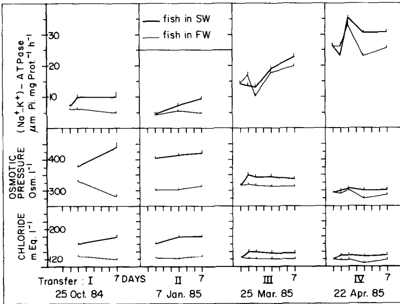
Fig. 3. Changes in osmotic parameters after four direct transfers to seawater in the Atlantic salmon (I, 25 October 1984; II, 7 January 1985; III, 25 March 1985; IV, 22 April 1985). Each point represents the mean ± the standard error of 10 fish.
