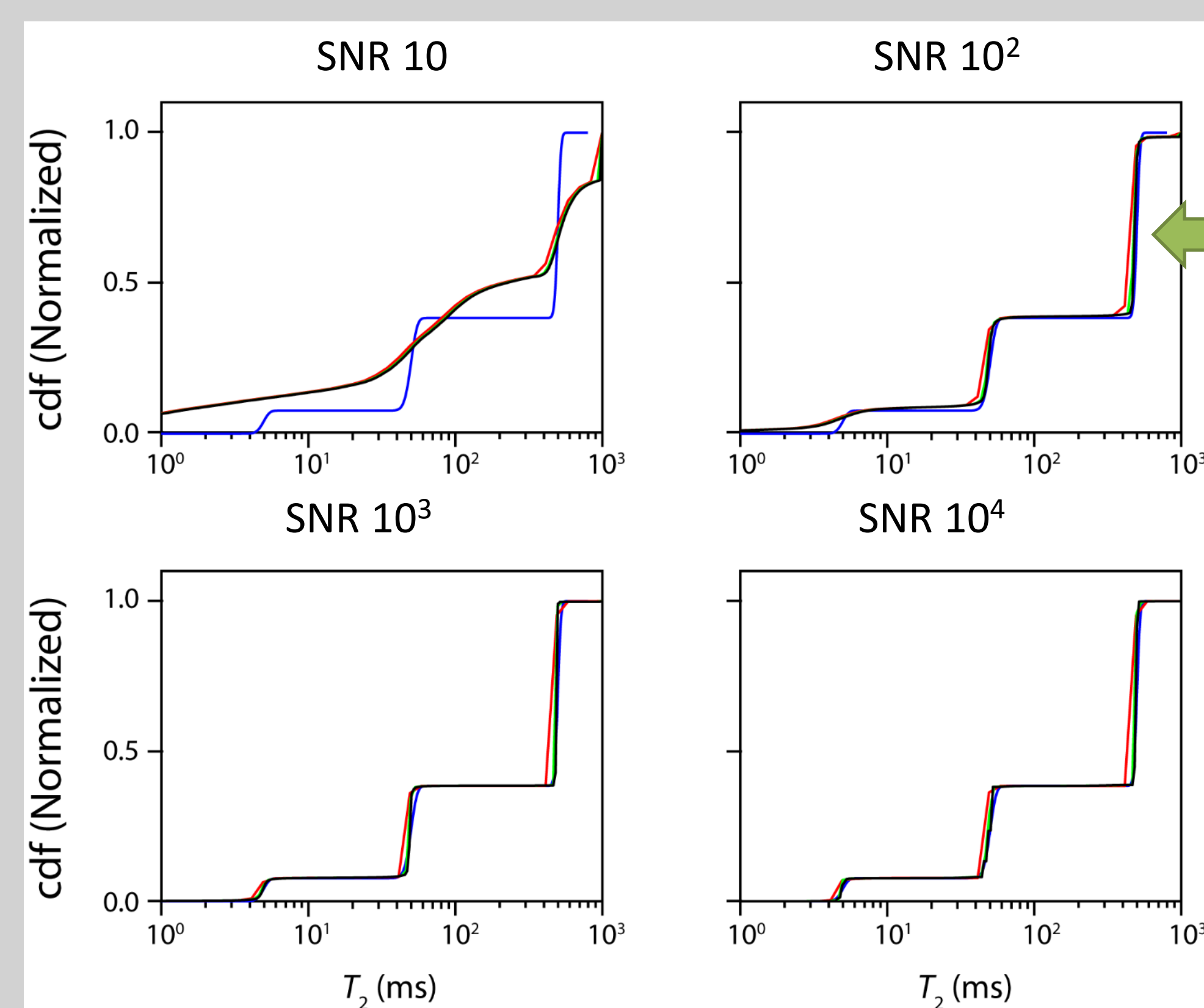
Figure 3: Averaged cdf results obtained from 10,000 NNLS analysis of noisy repetitions of the Gaussian model. The SNR was set to 10^1 , 10^2 , 10^3 and 10^4 . For both lowest SNRs, non-null amplitudes can be seen for the first point, i.e. edge artefacts.
