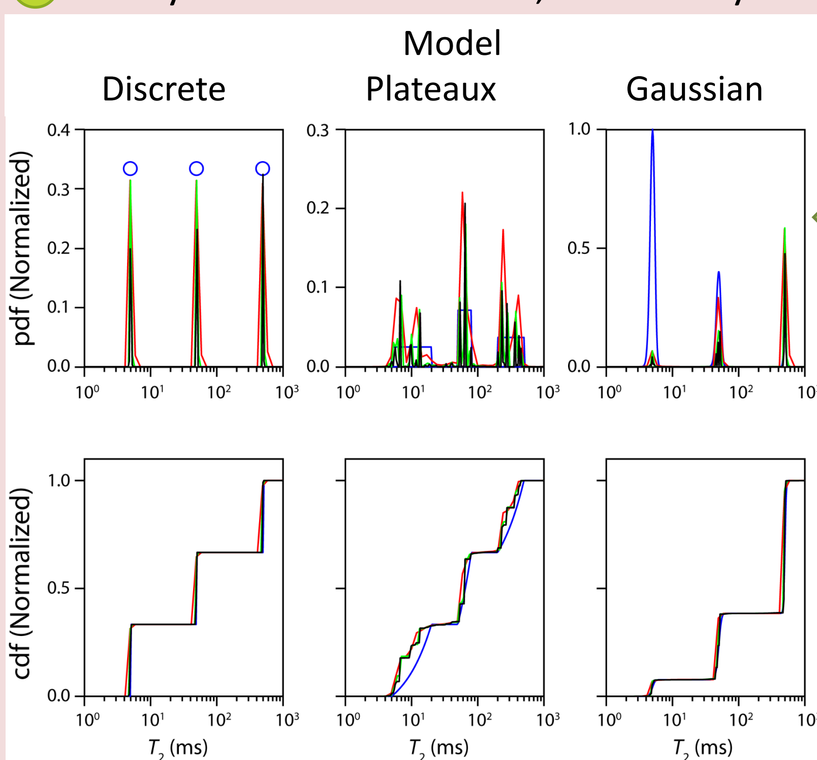
Figure 1: Averaged results for 10,000 simulated T_2 NMR signal decays (SNR 10^3 ) analysed with NNLS algorithm and a DB containing either 40 (blue) or 200 (red) T_2 values. Black lines represent the theoretical values. Representation as a pdf (top) and cdf (bottom).
